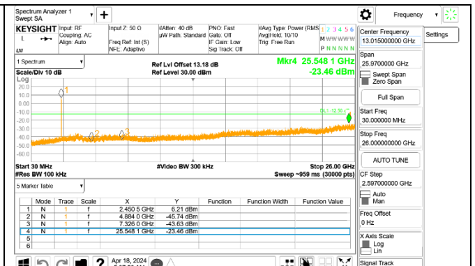
OUT-OF-BAND HIGH CHANNEL 7 Antenna 1
