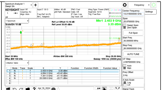
OUT-OF-BAND HIGH CHANNEL 8 Antenna 1
