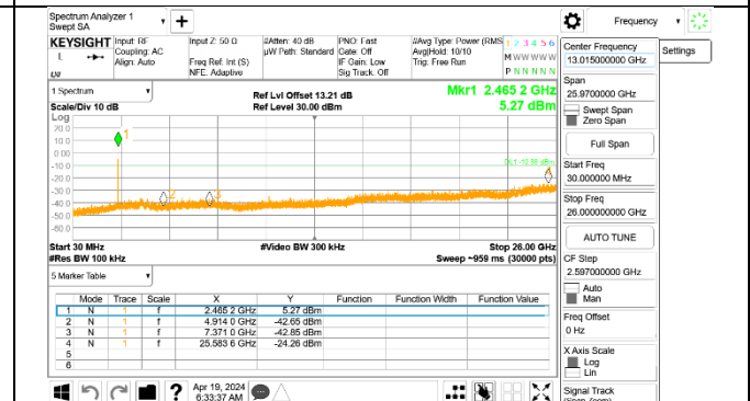
OUT-OF-BAND HIGH CHANNEL 10 Antenna 3
