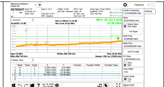
OUT-OF-BAND HIGH CHANNEL 11 Antenna 1
