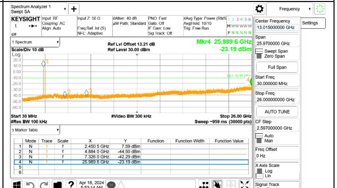
OUT-OF-BAND HIGH CHANNEL 7 Antenna 3
