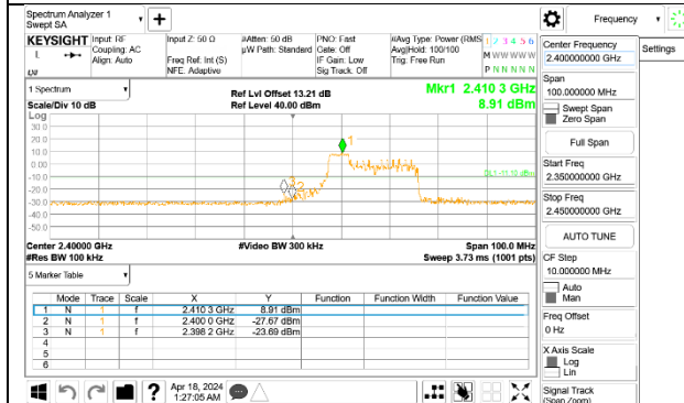
LOW CHANNEL 2 BANDEDGE Antenna 3
