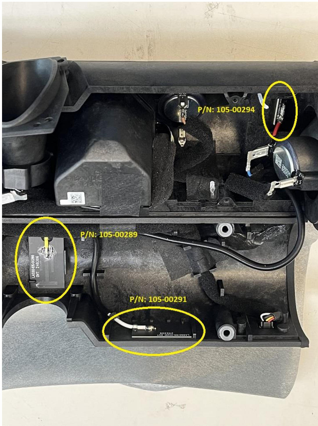
Photo 2: “Left Side” Antennas. P/N: 105-00294 Front Haul (FH) 5&6 GHz P/N: 105-00289 Back Haul (BH) 2.4, 5 & 6 GHz, P/N: 105-00291 BH 2.4, 5 & 6GHz
