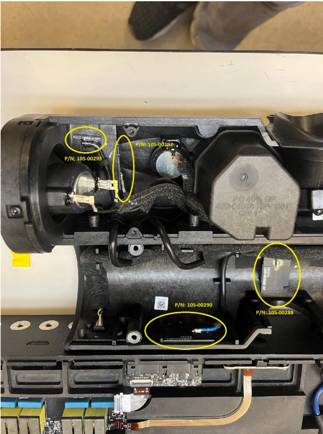
Photo 3: "Right Side" Antennas P/N: 105-00288 (BH) 2.4, 5 & 6 GHz, 105-00290 (BH) 2.4, 5 & 6 GHz, , P/N: 105-00292 (FH) 5&6 GHz, P/N: 105-00293 (FH) 5 & 6 GHz
