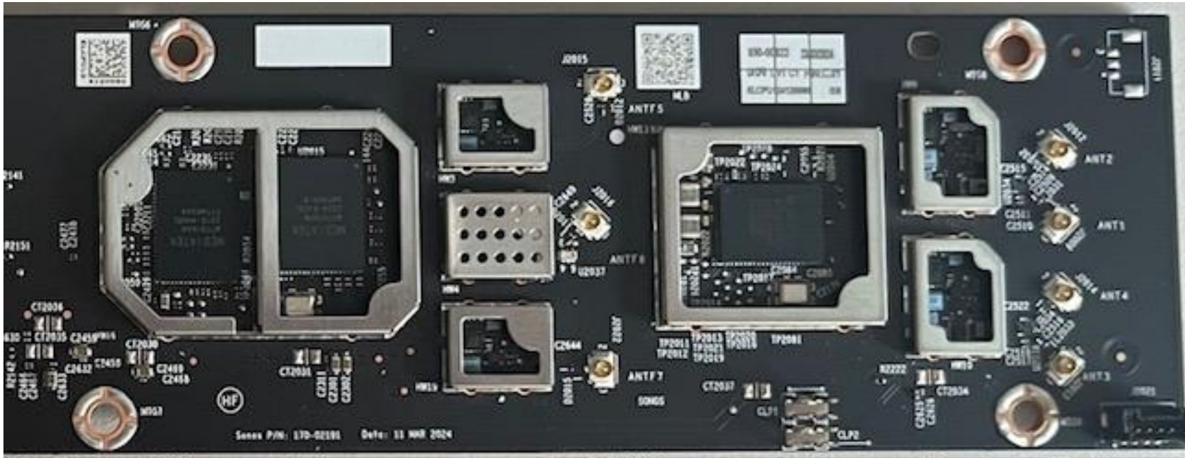
Photo 6: Close up of RF Section top of PCB.
