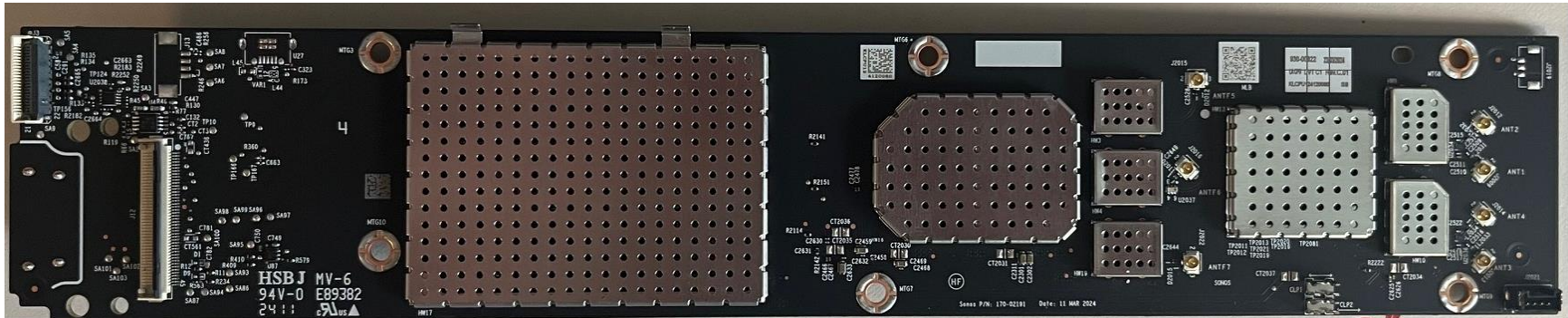
Photo 4: S45 CPU/RF PCB with RF Shields
