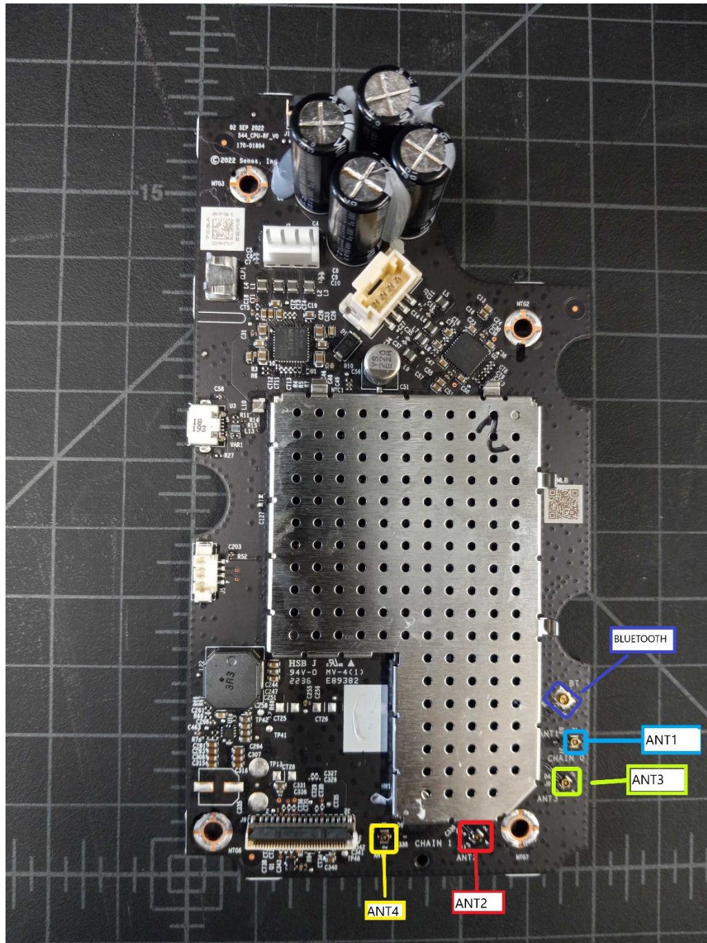
Main CPU/Radio board showing the radio connection ports.
