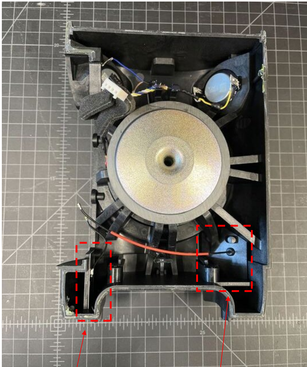
WiFi Antenna Chain 0 – ANT3
