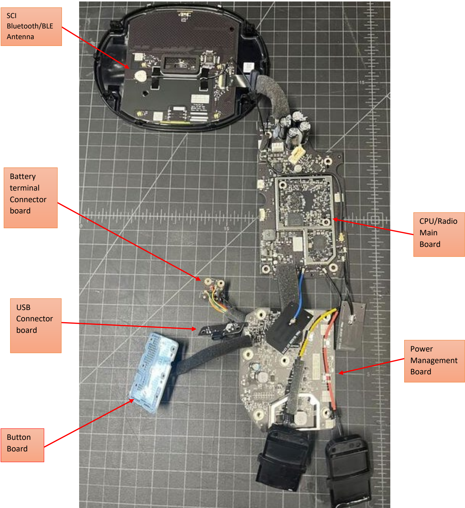
Main board, SCI board, Button Board, and power board assembly vie
