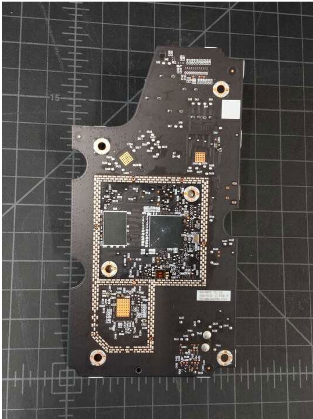
Main CPU/Radio board Bottom View
