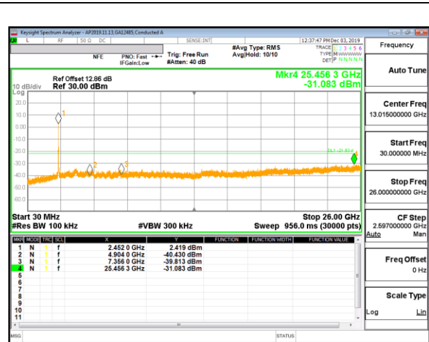
OUT-OF-BAND HIGH CHANNEL 9 CHAIN 0
