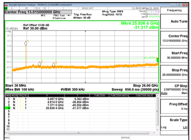
OUT-OF-BAND HIGH CHANNEL 10 CHAIN 3
