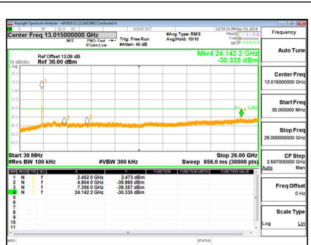
OUT-OF-BAND HIGH CHANNEL 9 CHAIN 3
