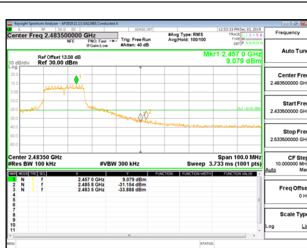
HIGH CHANNEL 9 BANDEDGE CHAIN 3
