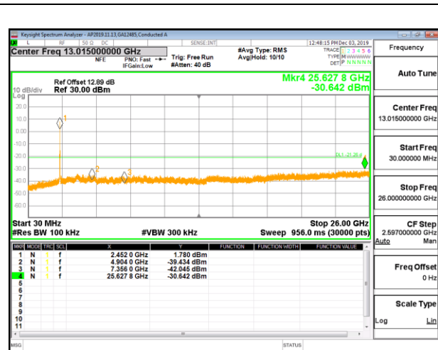
OUT-OF-BAND HIGH CHANNEL 9 CHAIN 2
