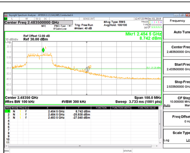
HIGH CHANNEL 9 BANDEDGE CHAIN 2
