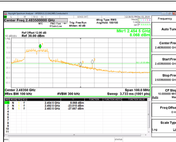
HIGH CHANNEL 9 BANDEDGE CHAIN 0
