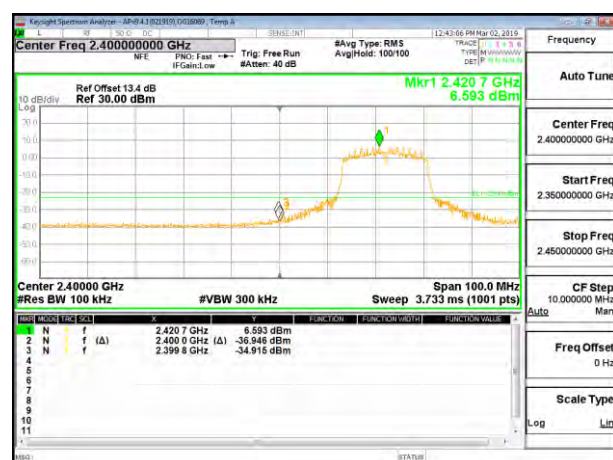
LOW CHANNEL 3 BANDEDGE CHAIN 3
