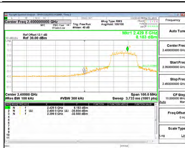
LOW CHANNEL 4 BANDEDGE CHAIN 2
