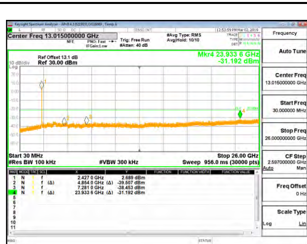
OUT-OF-BAND LOW CHANNEL 4 CHAIN 2
