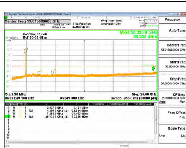
OUT-OF-BAND LOW CHANNEL 4 CHAIN 3
