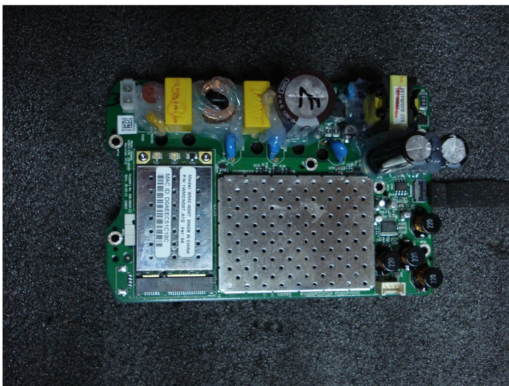
Main PCB top with shield
