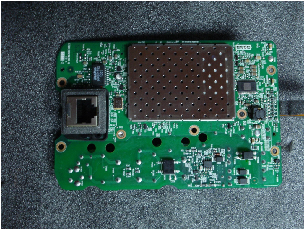
Main PCB bottom with shield
