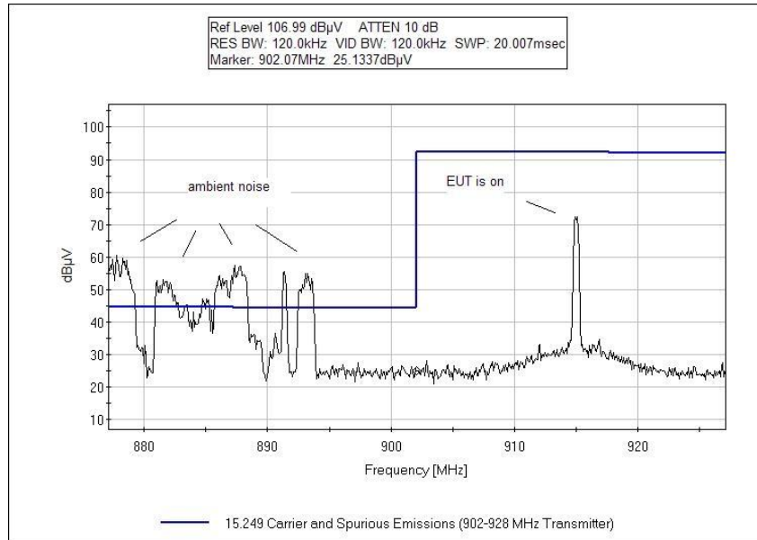
Left Bandedge with Tx On
