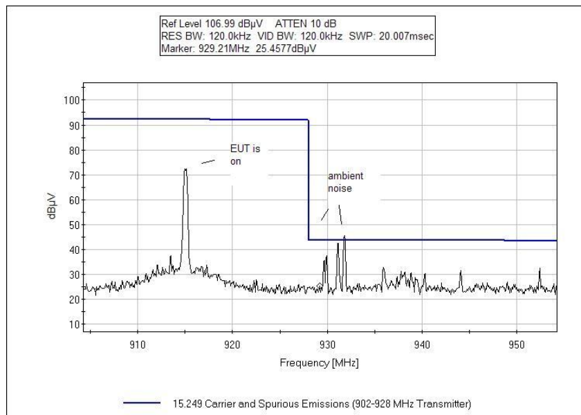
Right Bandedge with Tx On
