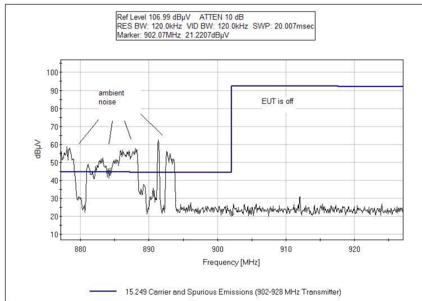
Left Bandedge with Tx Off
