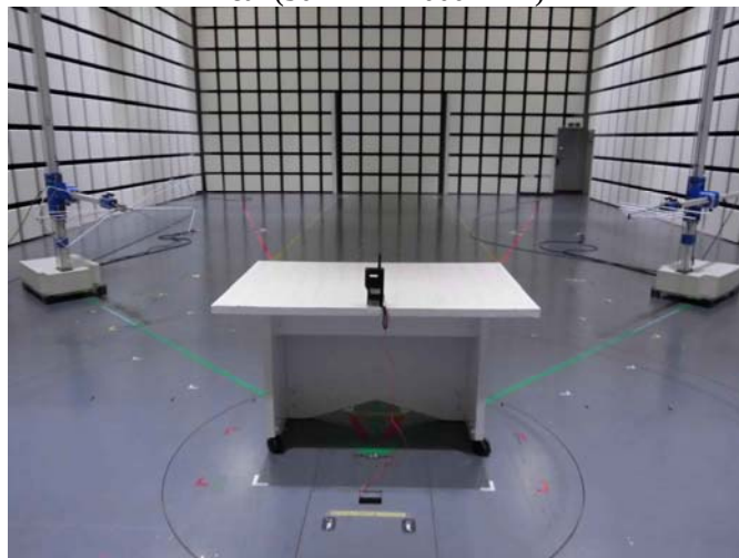
Rear (30 MHz - 1000 MHz)
