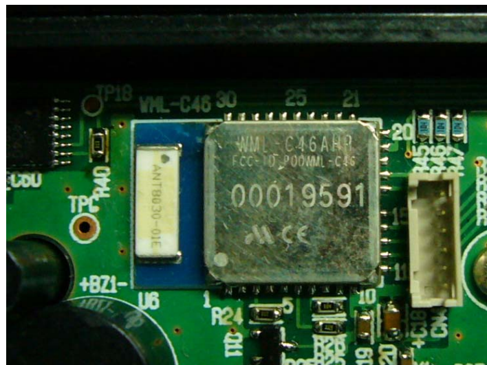
Bluetooth Module(Chip Ceramic Antenna) View
