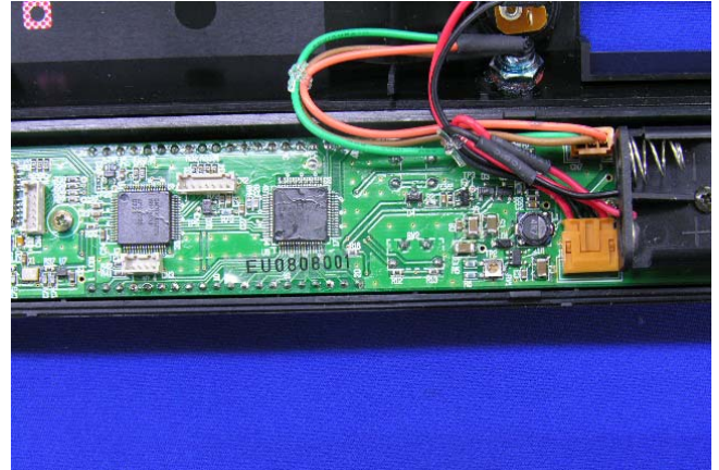
PCB(TOP) RIGHT View
