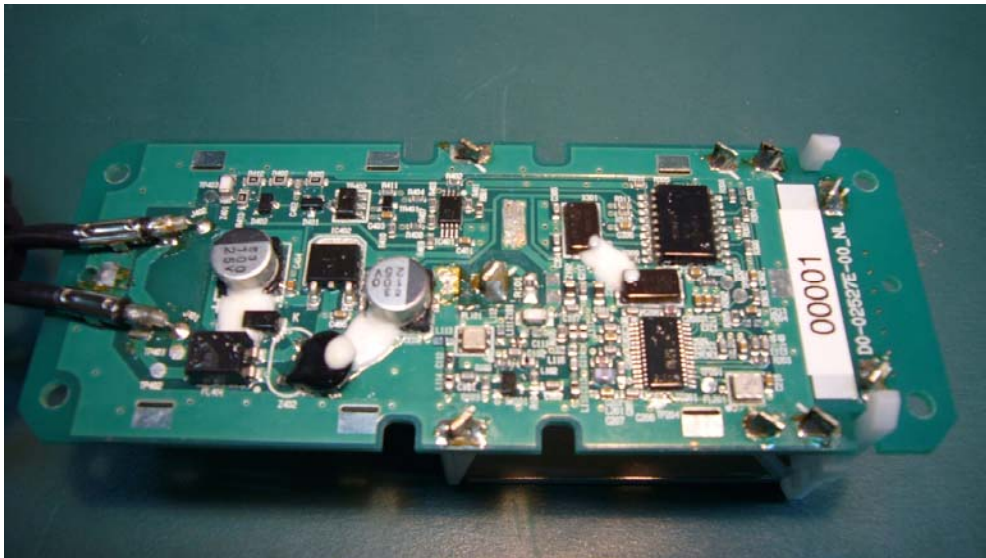
PCB View 1
