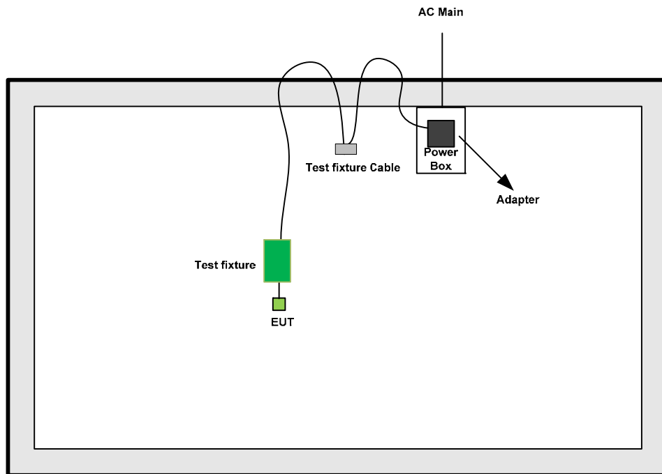
Test Setup Diagram –Radiated Emission > 1GHz
