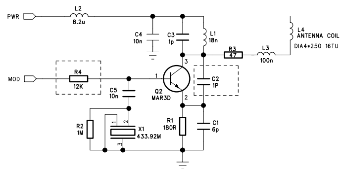
UHF TRANSMITTER
