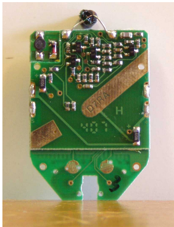
PCB (DC10r, computer)
