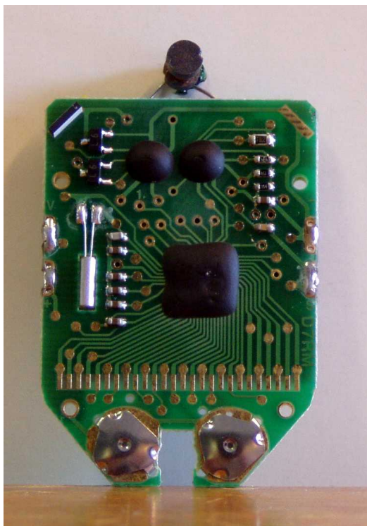
PCB (DC10r, computer)
