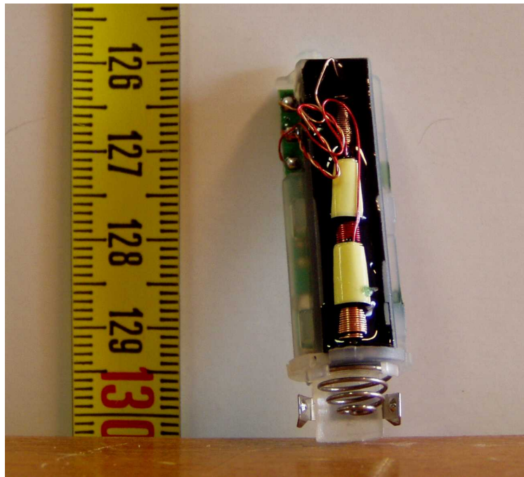
Transmitter
