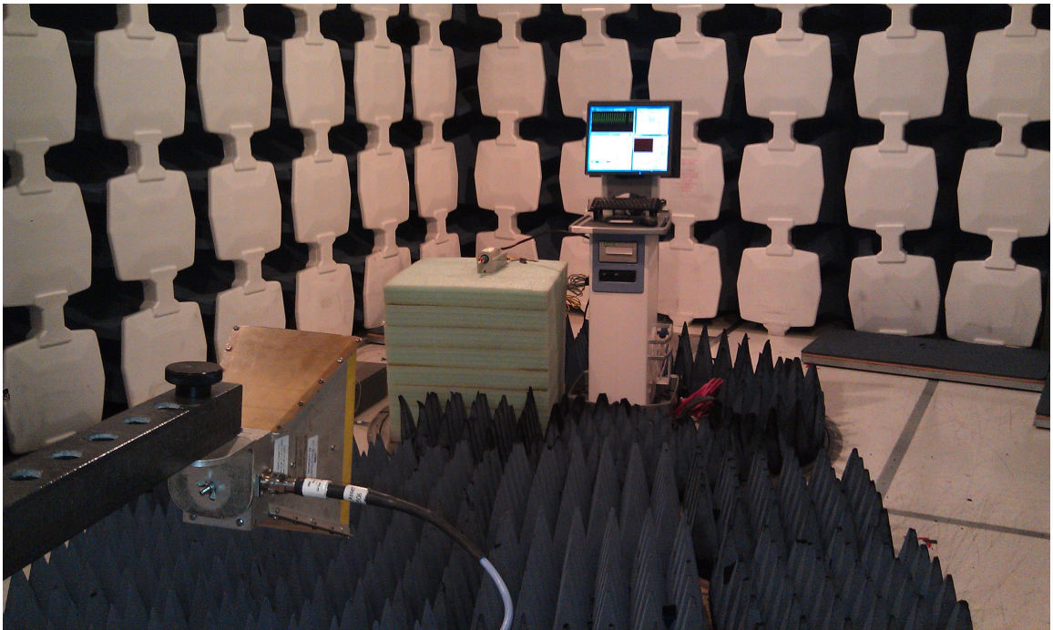
Emissions above 1GHz
