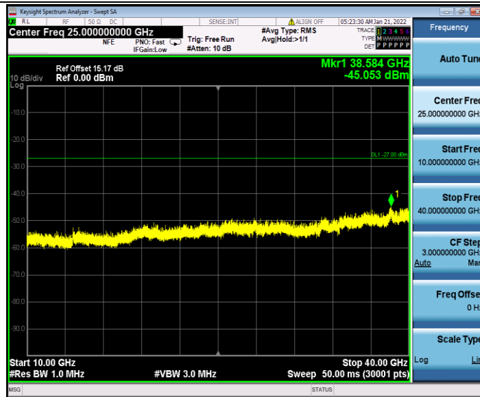
11AX40SISO_Ant2_7085_30~3000
