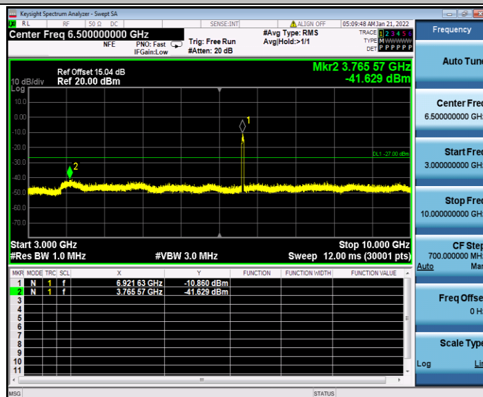
11AX40SISO_Ant1_6925_3000~10000
