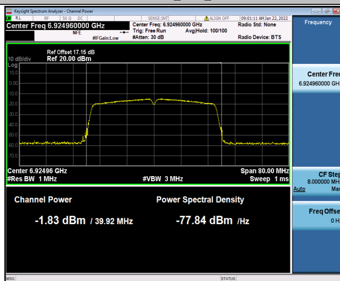
11N40SISO_Ant1_6925
