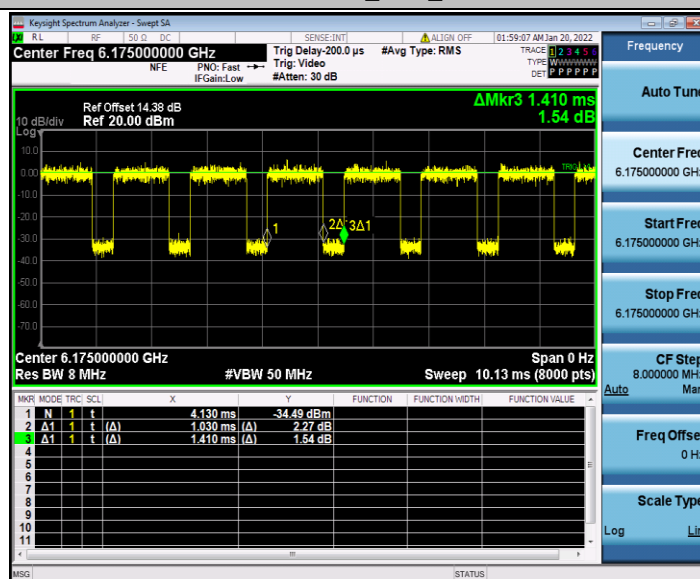
11AX20SISO_Ant1_6175
