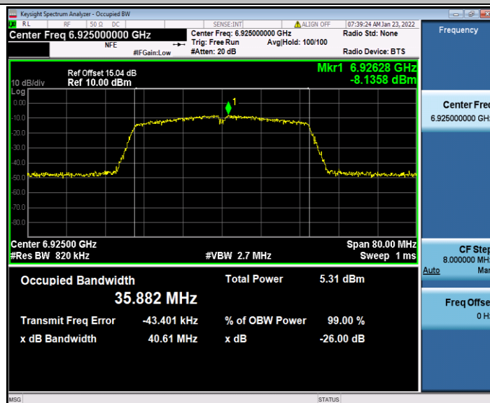
11AC40SISO_Ant1_6925
