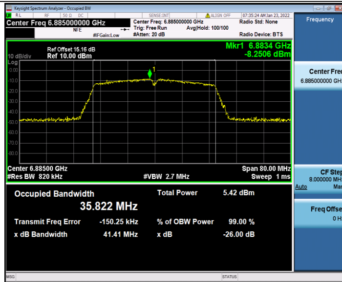
11AC40SISO_Ant2_6885
