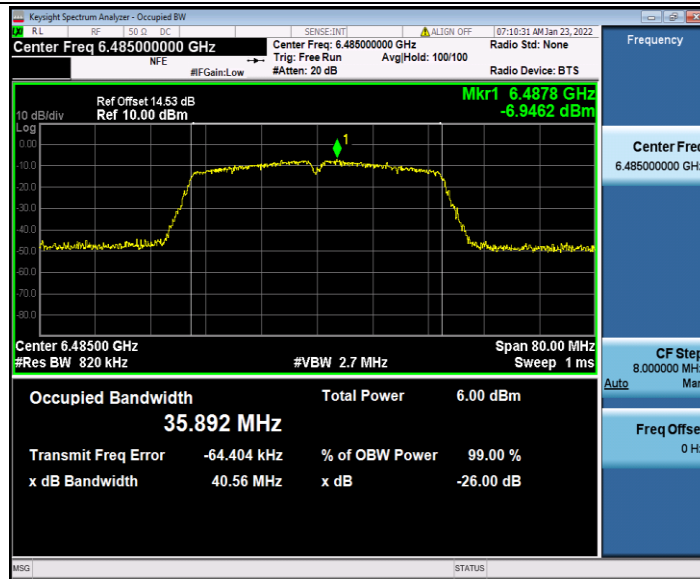
11AC40SISO_Ant2_6485
