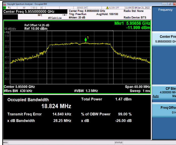
11N20SISO_Ant2_5955
