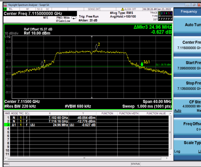
11AC20SISO_Ant2_7115
