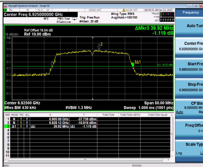
11N40SISO_Ant1_6925
