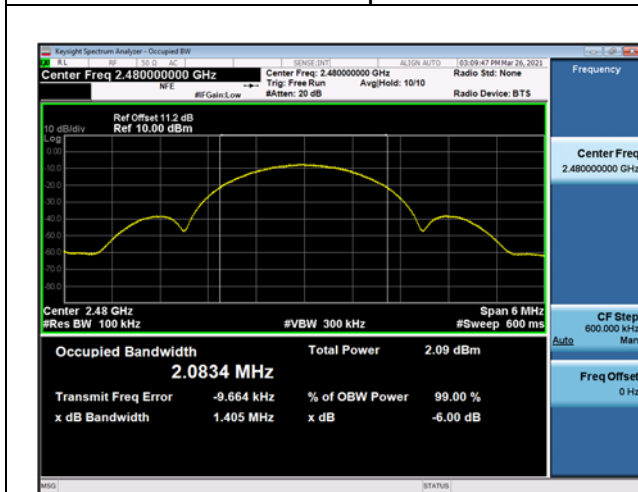
Modulation: 2Mbps 2480MHz
