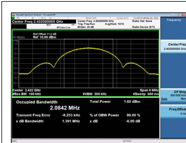
Modulation: 2Mbps 2402MHz
