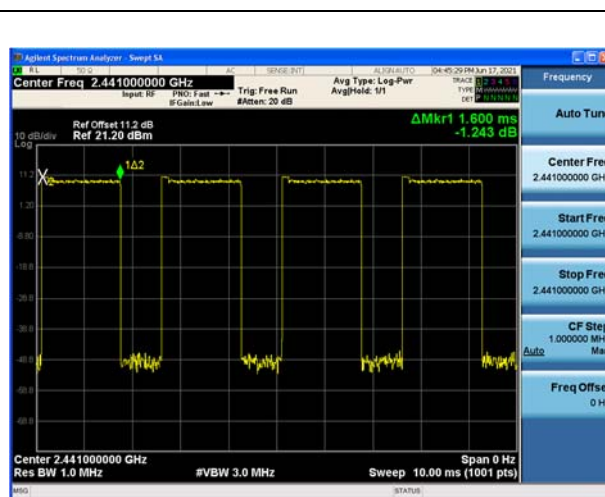
Modulation: 8DPSK DH3 2441
