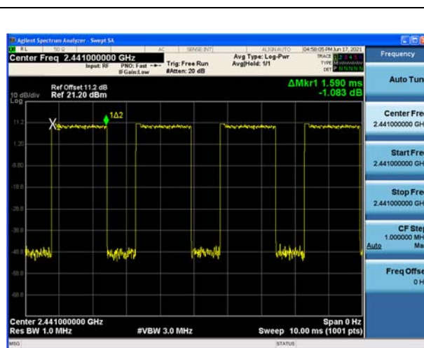
Modulation: \pi 4DQPSK DH3 2441
