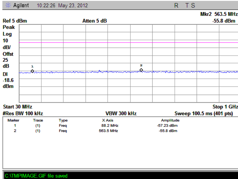
(Plot A.1: Channel = 0, 30MHz to 1GHz @ GFSK Mode)
