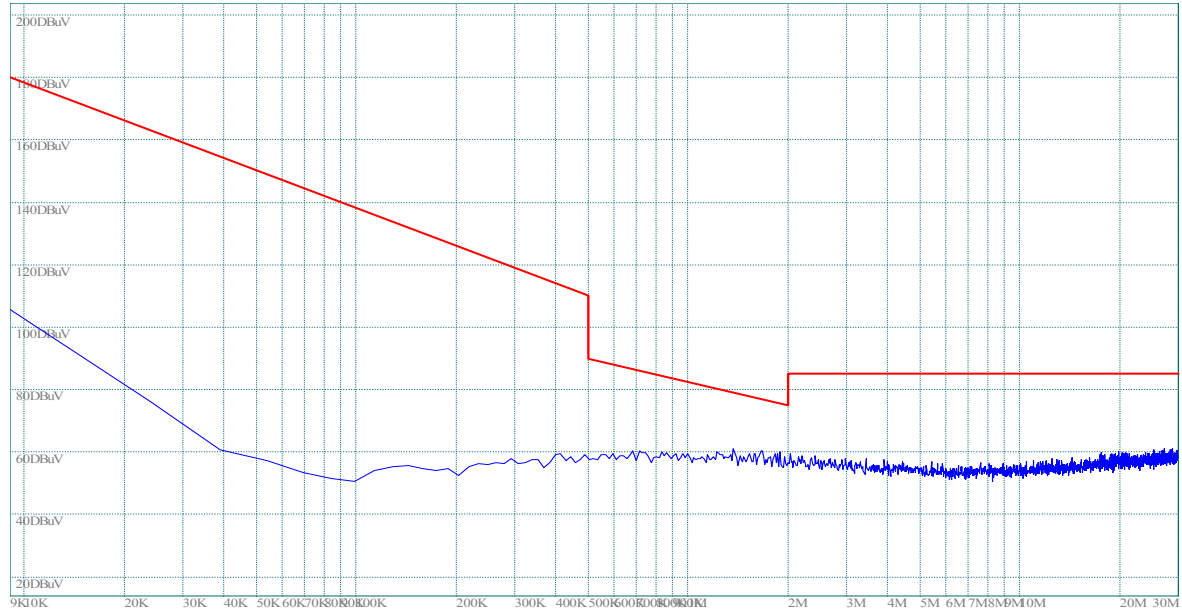
(Plot C.0: 9kHz to 30MHz @ 1/4-DQPSK, channel 78)
