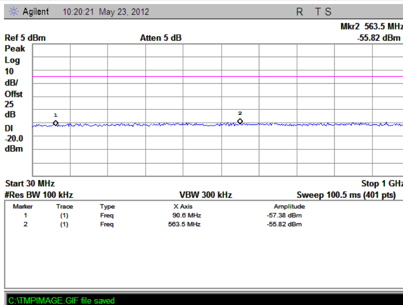
(Plot C.1: Channel = 78, 30MHz to 1GHz @ GFSK Mode)
