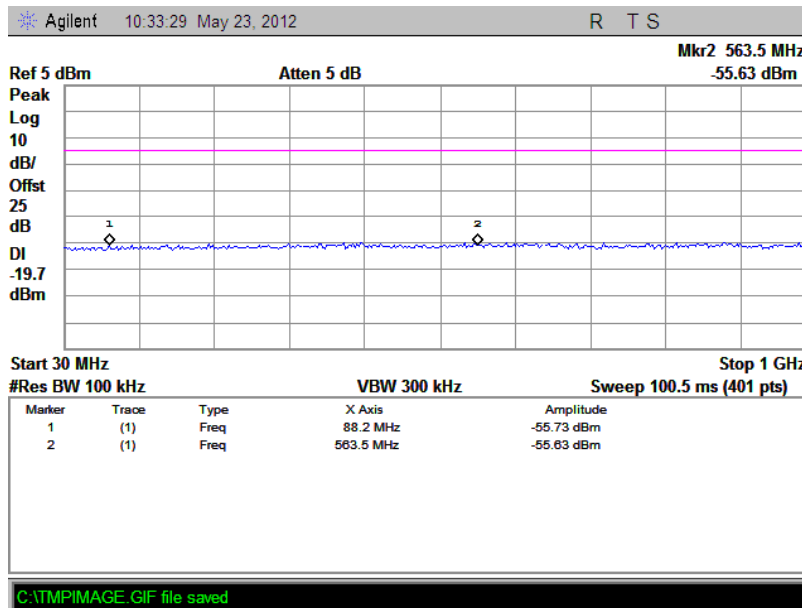
(Plot E.1: Channel = 39, 30MHz to 1GHz @ \pi/4 -DQPSK)
