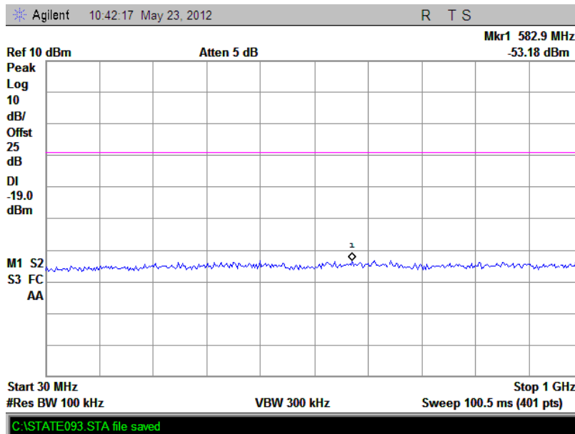
(Plot I.1: Channel = 78, 30MHz to 1GHz @ 8-DPSK)
