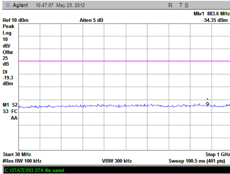
(Plot H.1: Channel = 39, 30MHz to 1GHz @ 8-DPSK)
