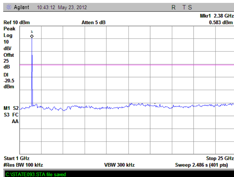
(Plot G.2: Channel = 0, 1GHz to 25GHz @ 8-DPSK)
