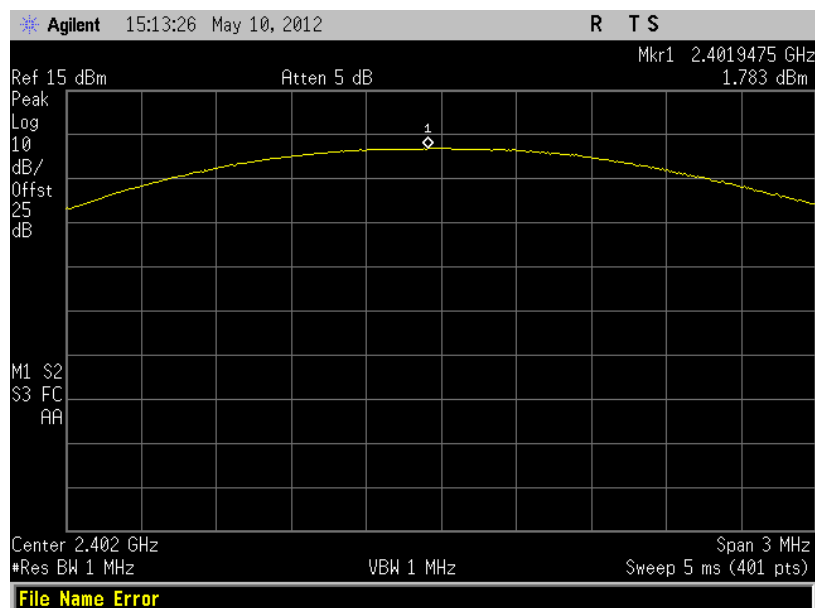
(Plot G: Channel = 2402 @ 8-DPSK)
