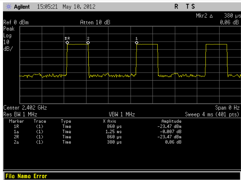
(Plot A: Channel = 2402 @ GFSK)
