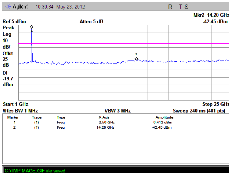
(Plot F.2: Channel = 78, 1GHz to 25GHz @ \pi/4 -DQPSK)
