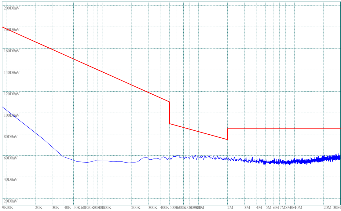
(Plot C.0: 9kHz to 30MHz @ 8-DPSK, channel 78)
