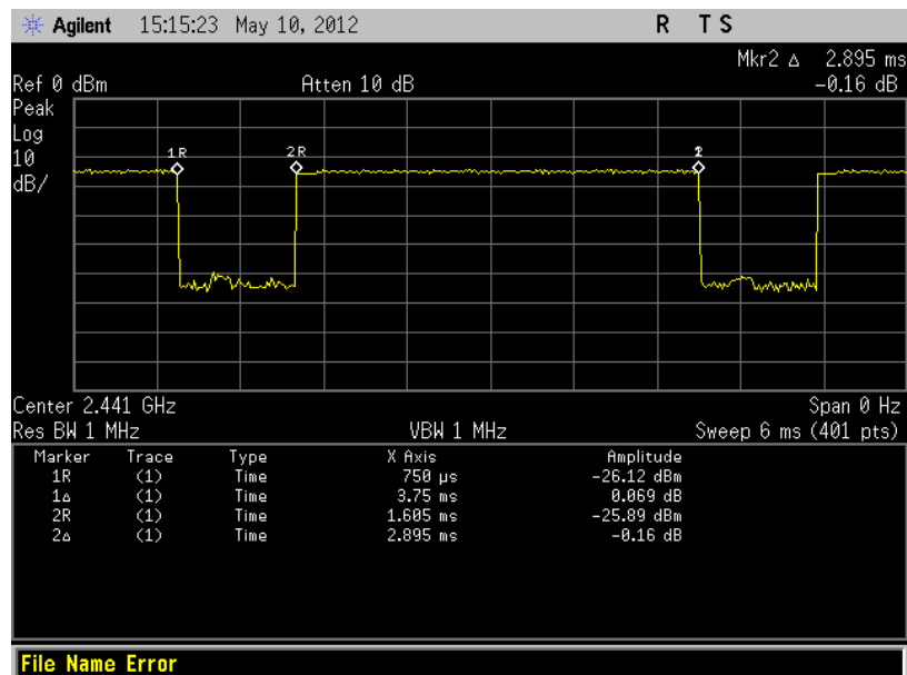
(Plot H: Channel = 2441 @ 8-DPSK)
