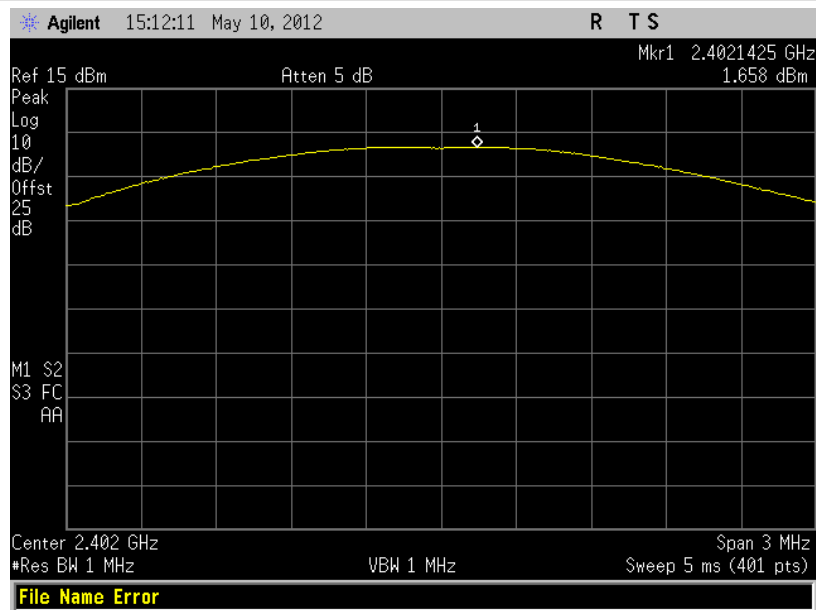
(Plot D: Channel = 2402 @ \pi/4 -DQPSK)
