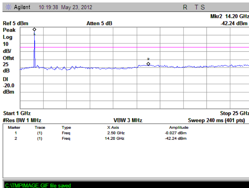
(Plot C.2: Channel = 78, 1GHz to 25GHz @ GFSK Mode)
