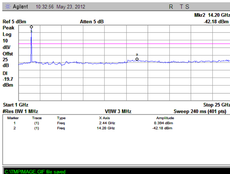
(Plot E.2: Channel = 39, 1GHz to 25GHz @ \pi/4 -DQPSK)
