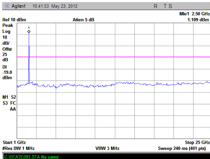
(Plot I.2: Channel = 78, 1GHz to 25GHz @ 8-DPSK)
