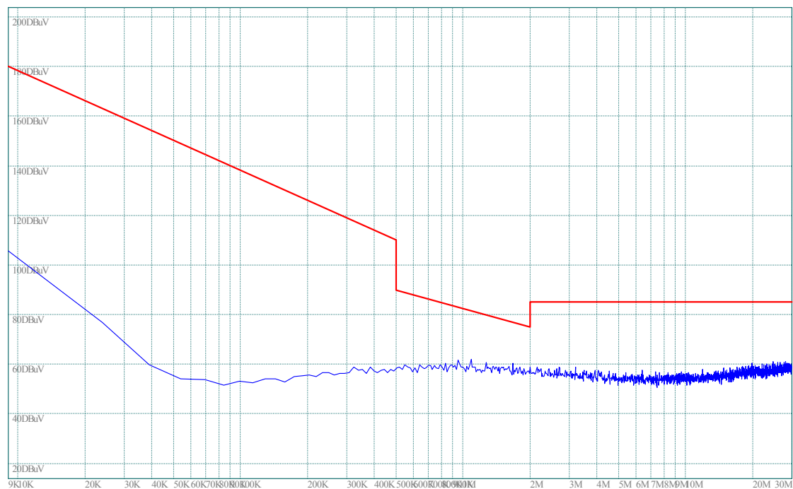
(Plot B.0: 9kHz to 30MHz @ 8-DPSK, channel 39)
