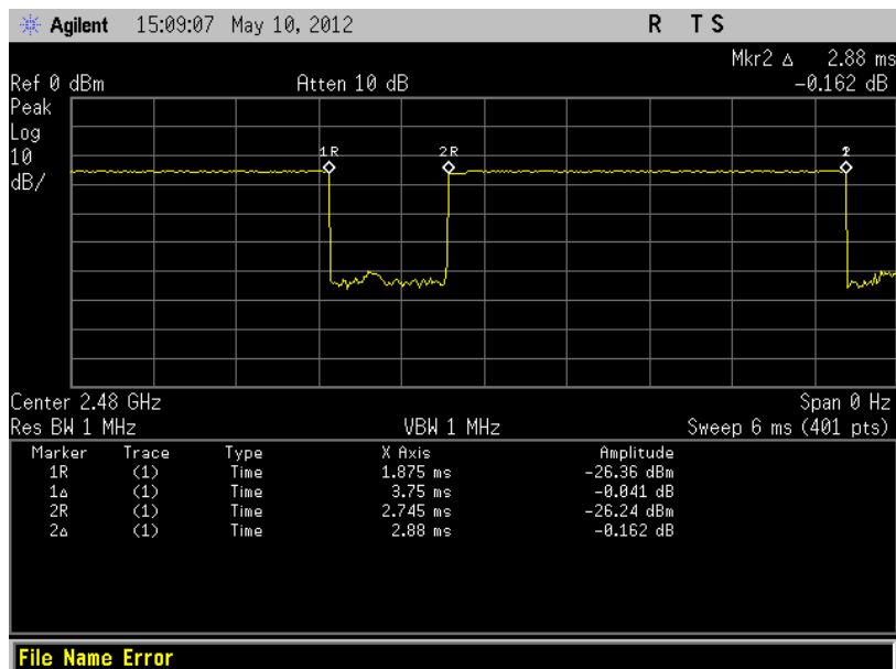
(Plot F: Channel = 2480 @ \pi/4 -DQPSK)
