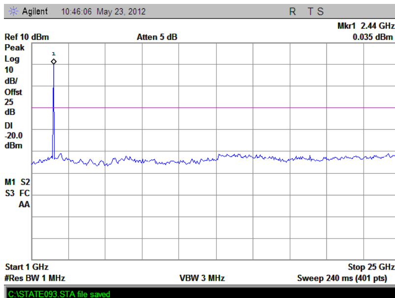
(Plot B.2: Channel = 39, 1GHz to 25GHz @ GFSK Mode)
