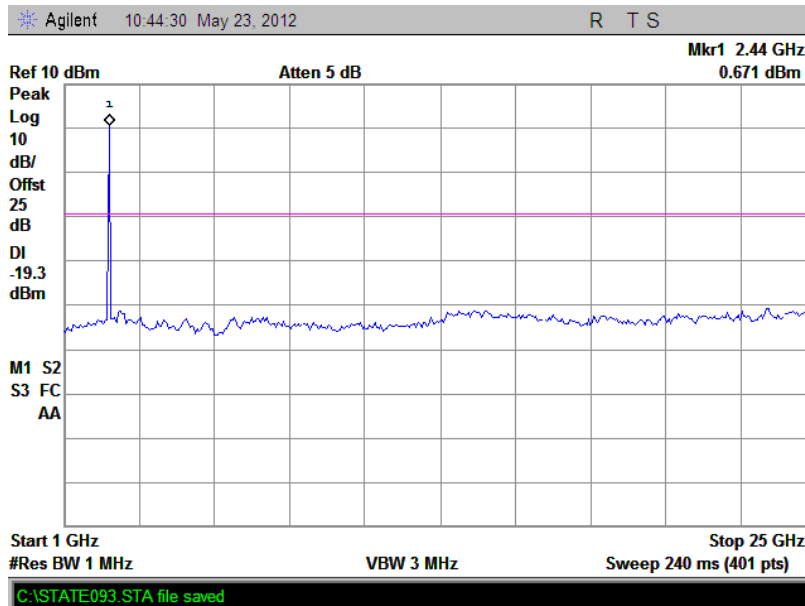
(Plot H.2: Channel = 39, 1GHz to 25GHz @ 8-DPSK)
