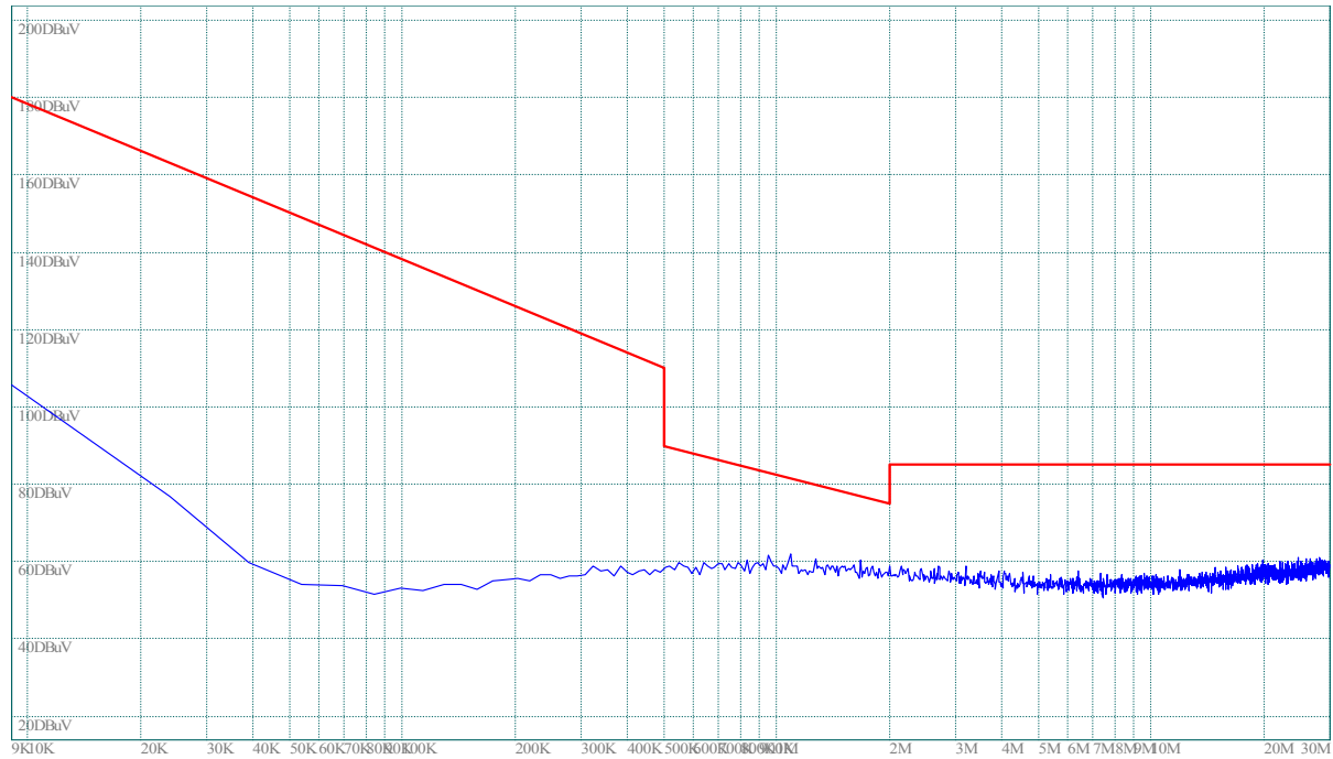
(Plot A.0: 9kHz to 30MHz @ 8-DPSK, channel 0)
