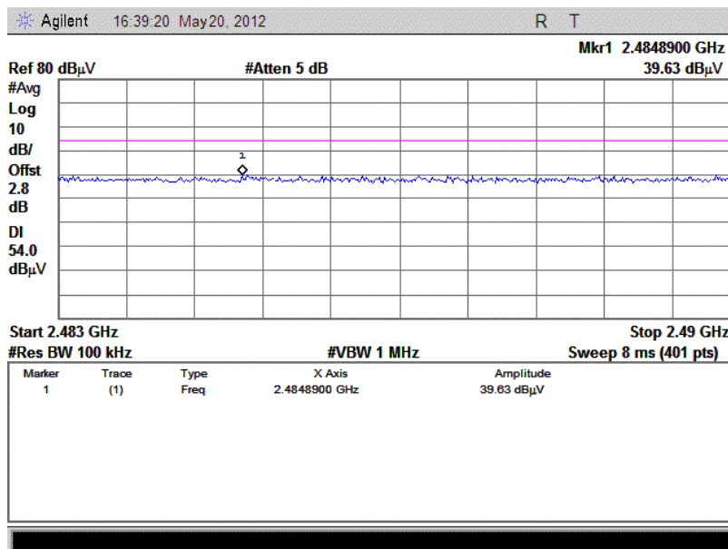
(Plot F2: Channel = 78 AVERAGE @ 8-DPSK Mode)
