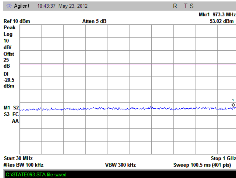
(Plot G.1: Channel = 0, 30MHz to 1GHz @ 8-DPSK)
