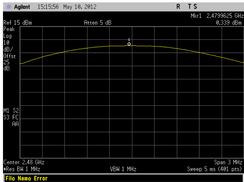
(Plot I: Channel = 2480 @ 8-DPSK)
