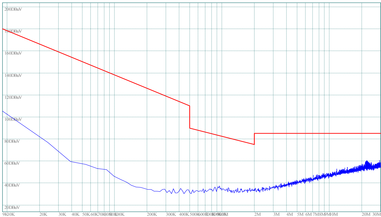
(Plot B.0: 9kHz to 30MHz @ GFSK, channel 39)
