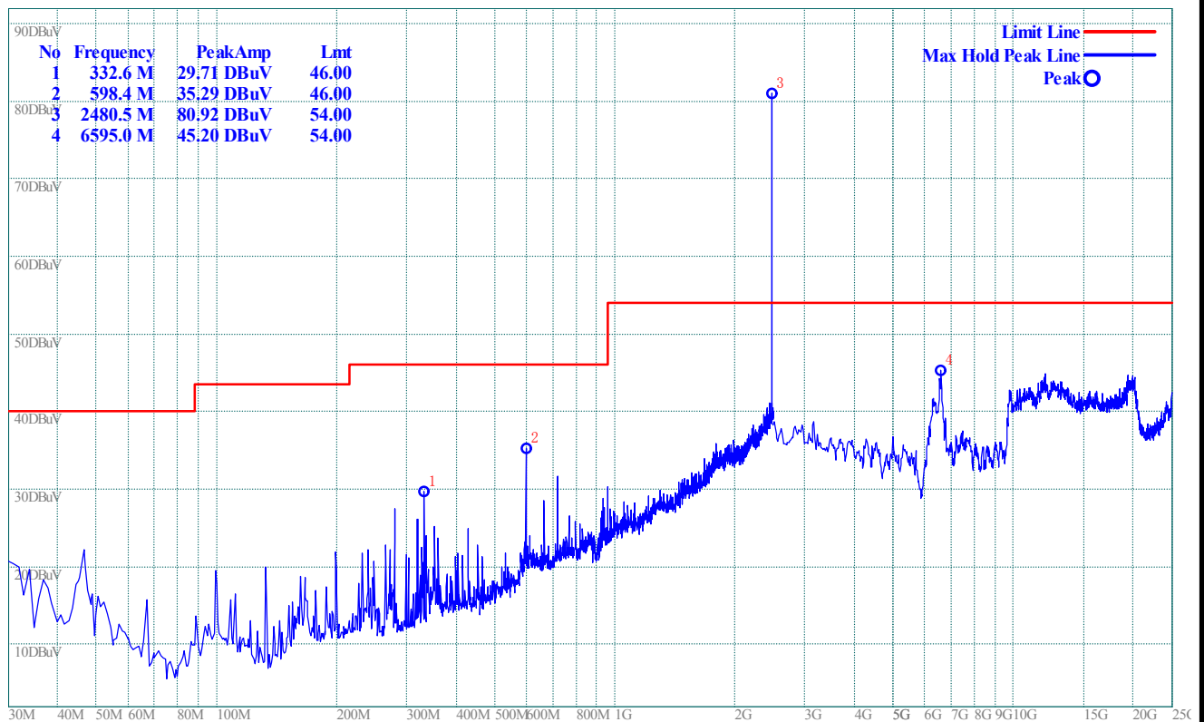
(Plot C.1: 30MHz to 25GHz, Antenna Horizontal @ 1/4-DQPSK, channel 78)
