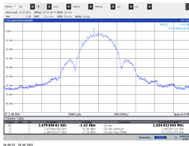
Figure 7.4-3: 99% occupied bandwidth on high channel
