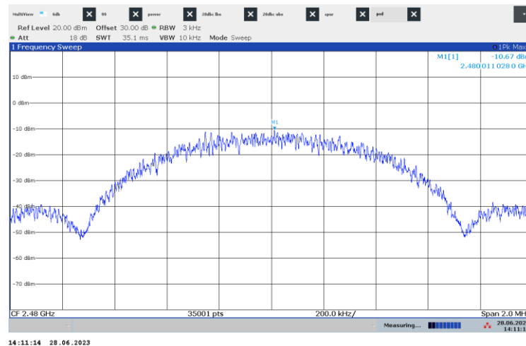
Figure 7.7-3: PSD on high channel
