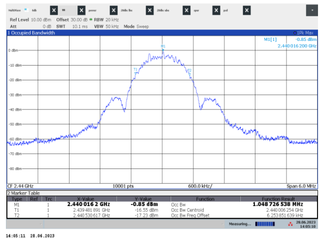
Figure 7.4-2: 99% occupied bandwidth on mid channel
