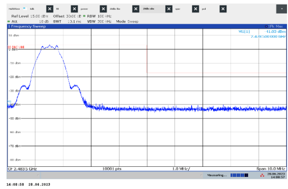
Figure 7.6-2: Out of band emissions at the upper band edge
