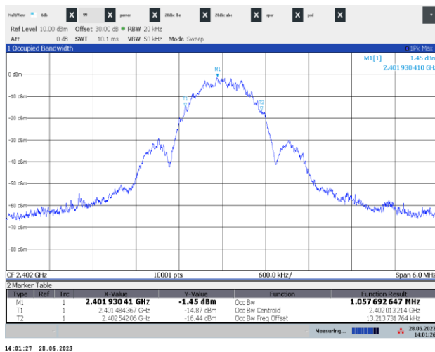
Figure 7.4-1: 99% occupied bandwidth on low channel
