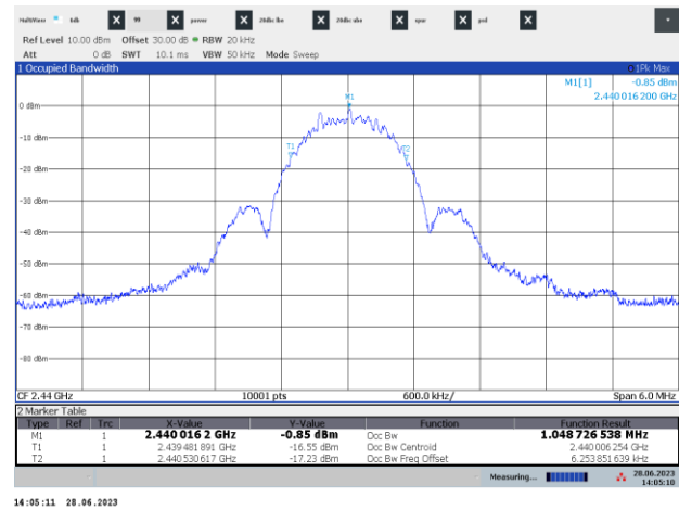
Figure 7.4-2: 99% occupied bandwidth on mid channel
