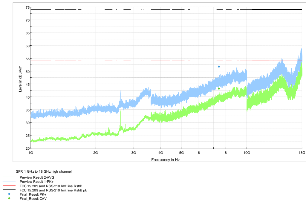
Figure 7.6-10: Spurious emissions above 1 GHz to 18 GHz, High channel
