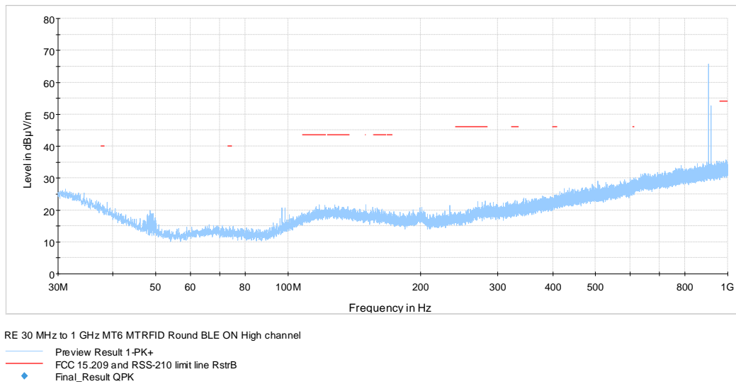
Figure 7.6-9: Spurious emissions below 1 GHz, High channel
