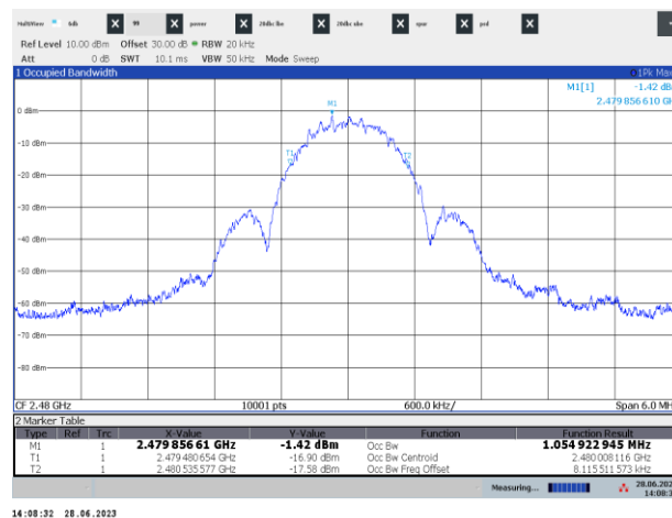
Figure 7.4-3: 99% occupied bandwidth on high channel
