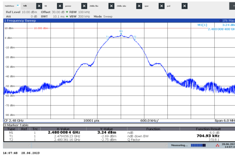
Figure 7.4-6: 6 dB bandwidth on high channel
