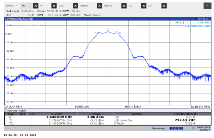
Figure 7.4-5: 6 dB bandwidth on mid channel
