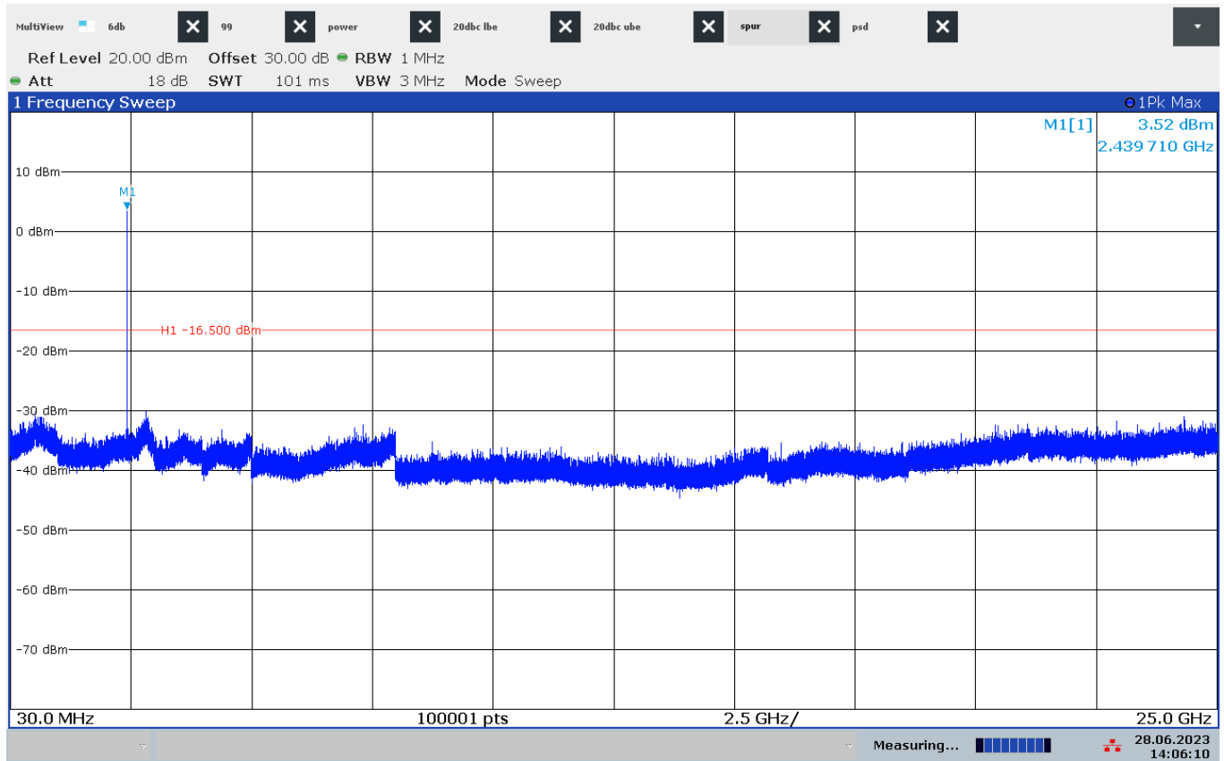
Figure 7.6-13: Spurious emissions 30 MHz to 25 GHz, mid channel
