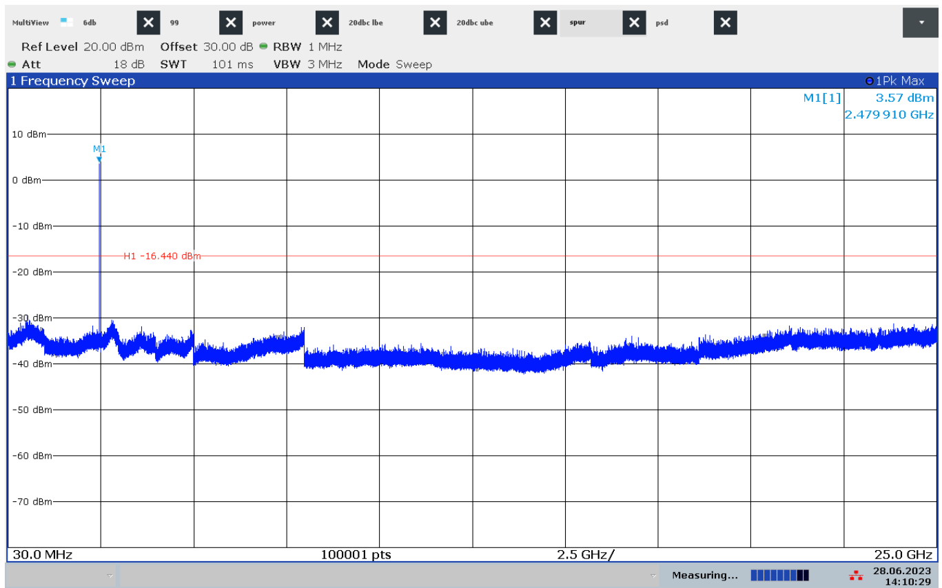
Figure 7.6-14: Spurious emissions 30 MHz to 25 GHz, high channel
