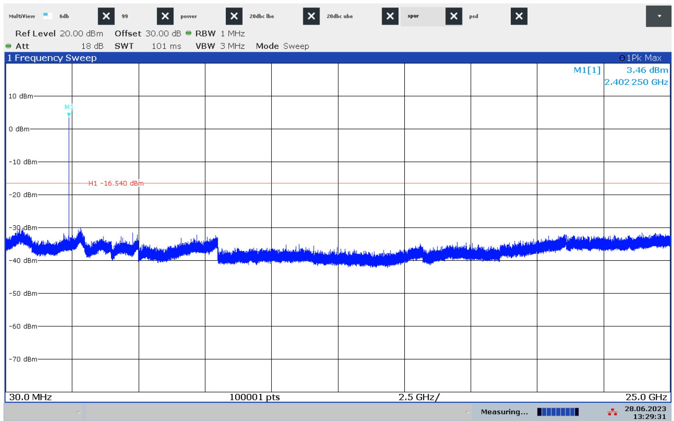
Figure 7.6-12: Spurious emissions 30 MHz to 25 GHz, low channel
