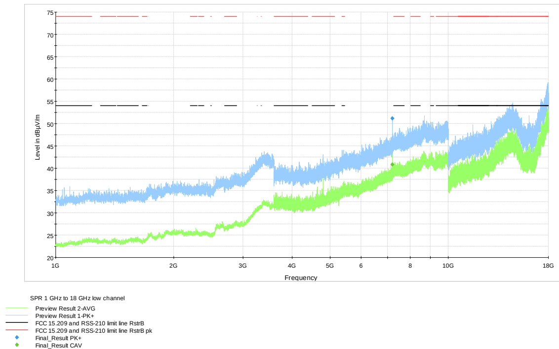
Figure 7.6-4: Spurious emissions 1 GHz to 18 GHz, low channel
