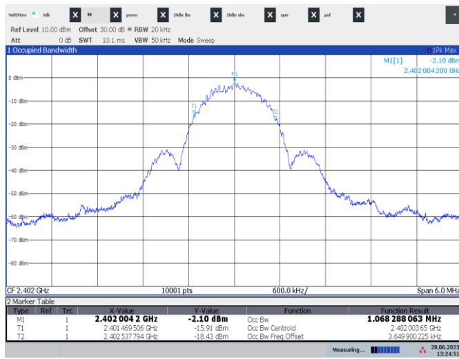
Figure 7.4-1: 99% occupied bandwidth on low channel
