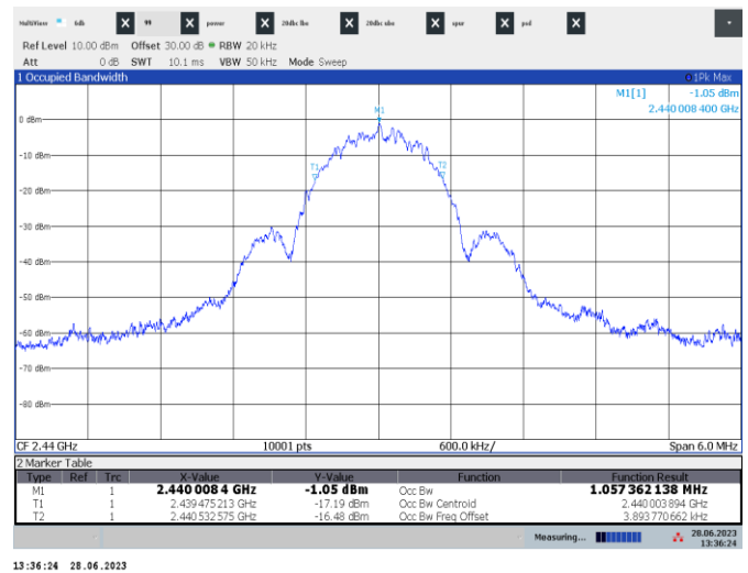
Figure 7.4-2: 99% occupied bandwidth on mid channel
