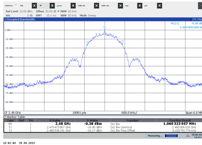
Figure 7.4-3: 99% occupied bandwidth on high channel
