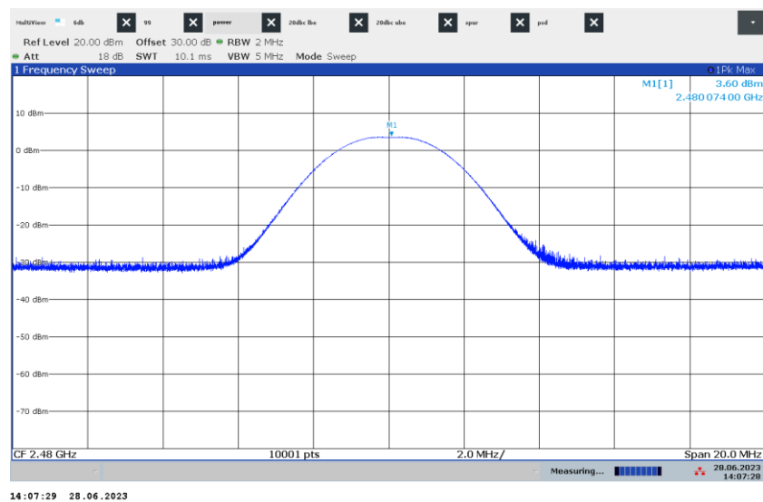
Figure 7.5-3: Output power on high channel
