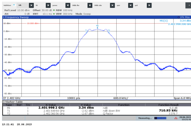
Figure 7.4-4: 6 dB bandwidth on low channel
