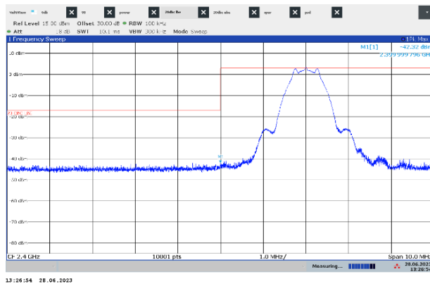
Figure 7.6-1: Out of band emissions at the lower band edge
