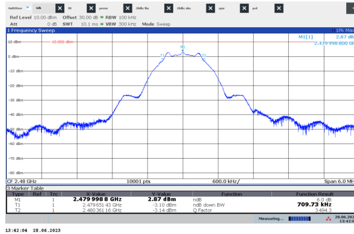
Figure 7.4-6: 6 dB bandwidth on high channel
