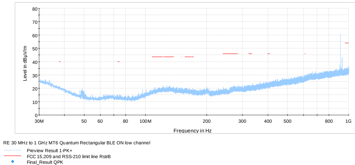
Figure 7.6-3: Spurious emissions below 1 GHz, low channel
