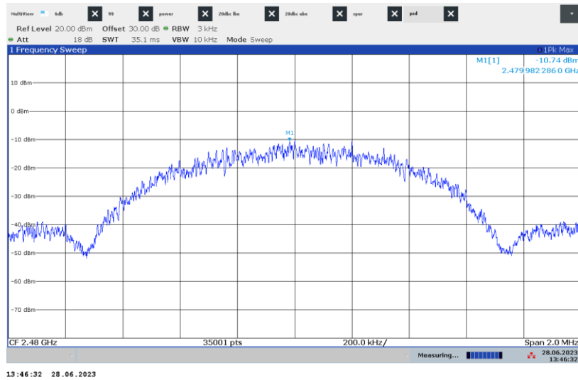
Figure 7.7-3: PSD on high channel
