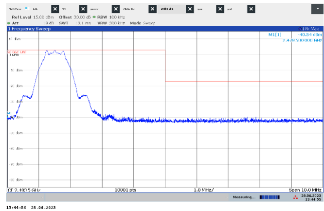
Figure 7.6-2: Out of band emissions at the upper band edge
