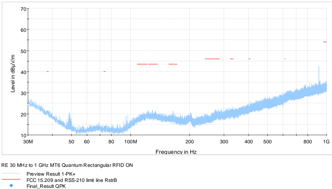
Figure 7.6-2: Field strength of spurious emissions above 30 MHz
