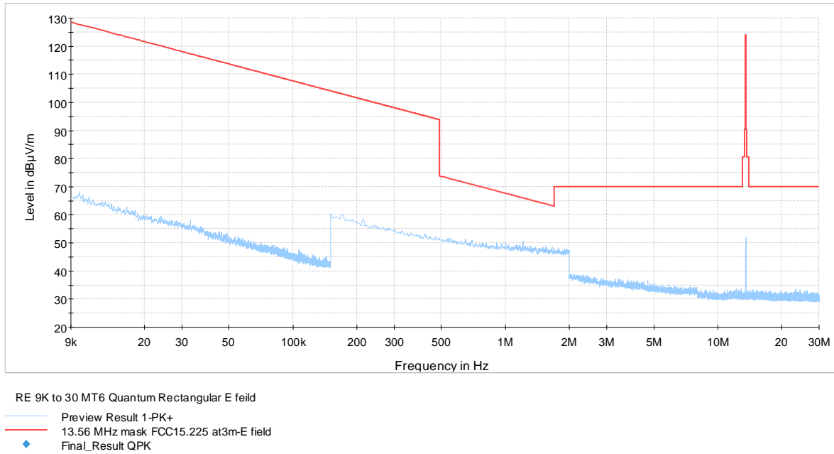
Figure 7.6-1: Field strength of spurious emissions below 30 MHz
