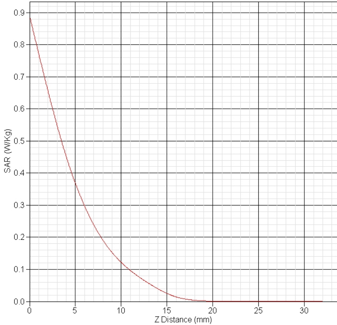
SAR-Z Axis at Hotspot x:0.08 y:7.91
