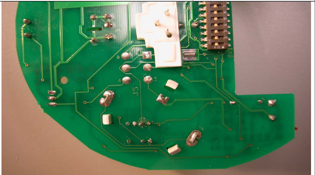
PCB 2 Back Component
