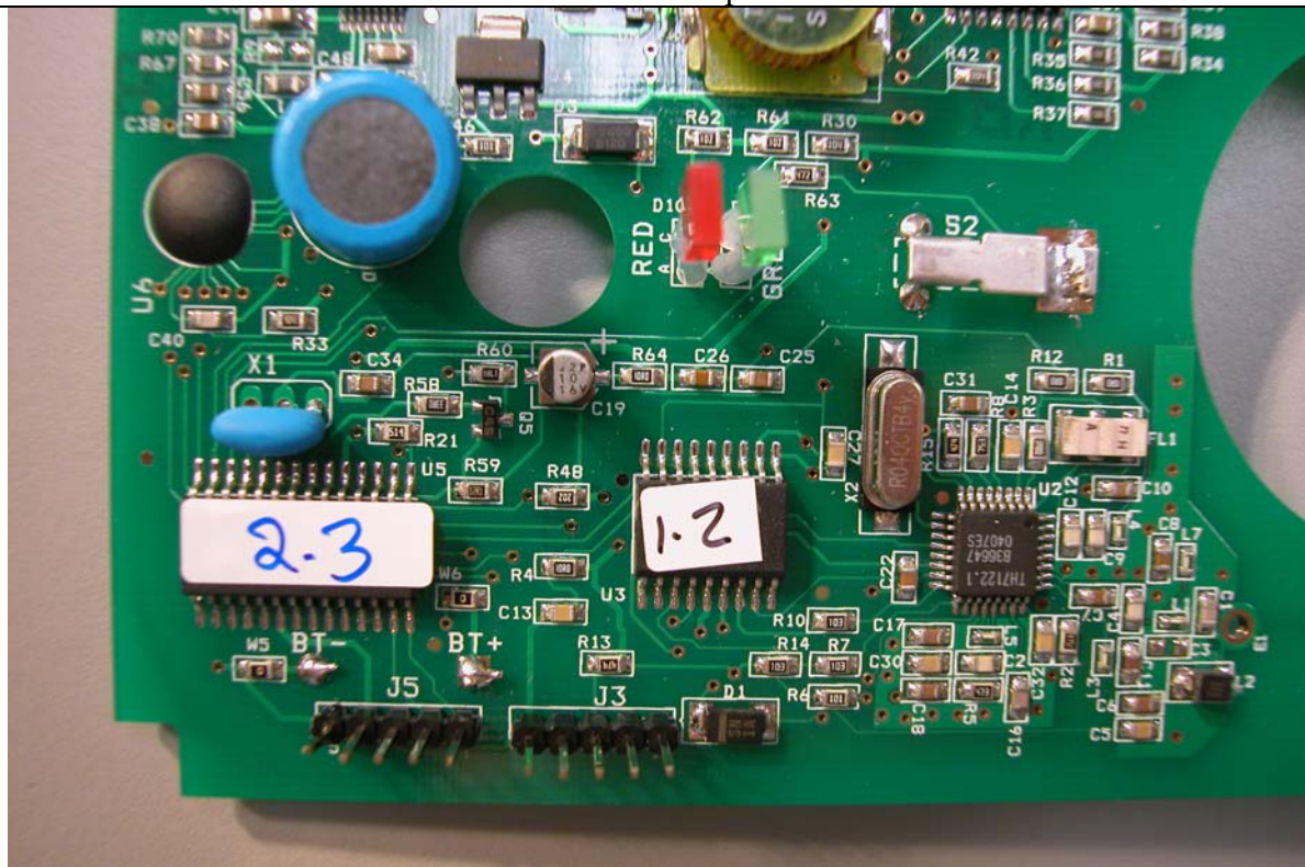
PCB front 3 Components
