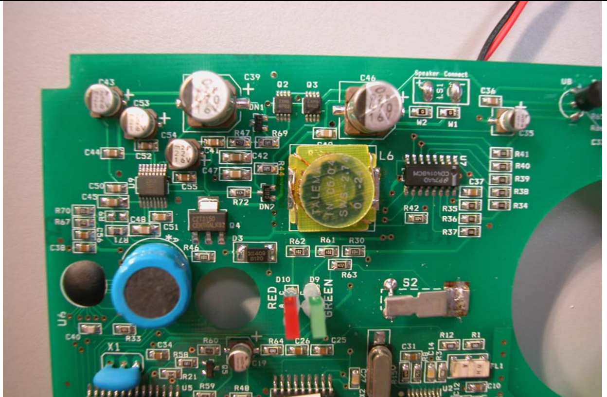
PCB 1front Components
