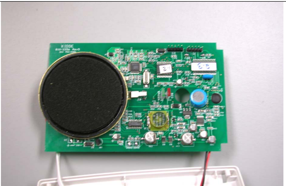
Top half of PCB
