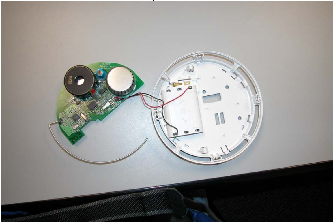
PCB removed
