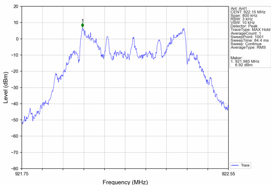
915Mhz_HCH_922.15MHz_Ant1_NTNV
