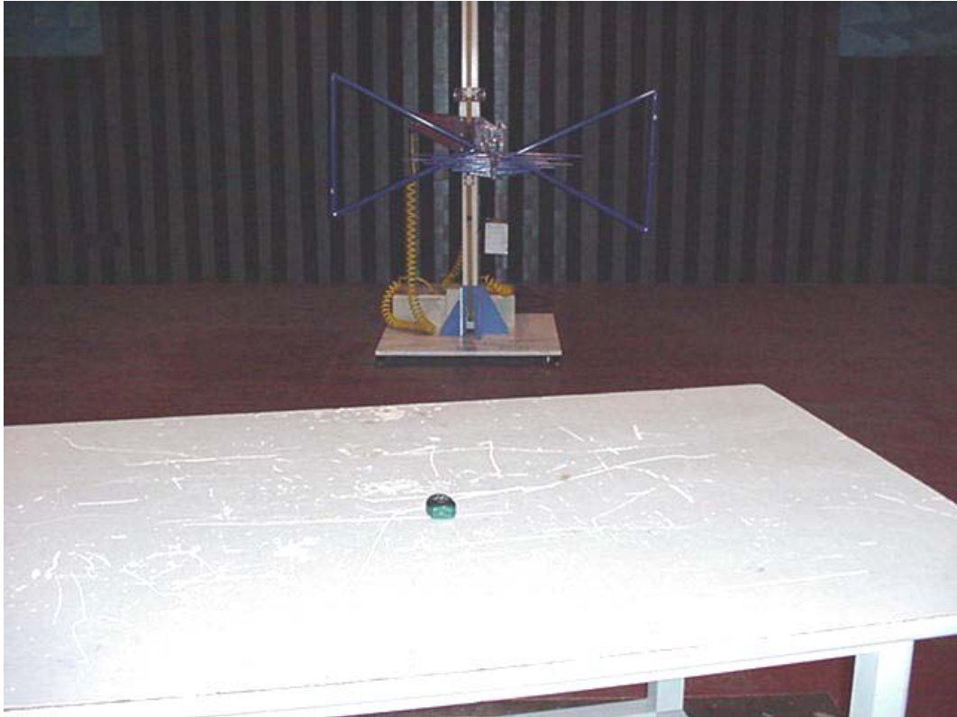
SETUP WITH MAXIMUM DETECTED EMISSION AT HORIZONTAL POLARIZATION (2 TEST MODE)
