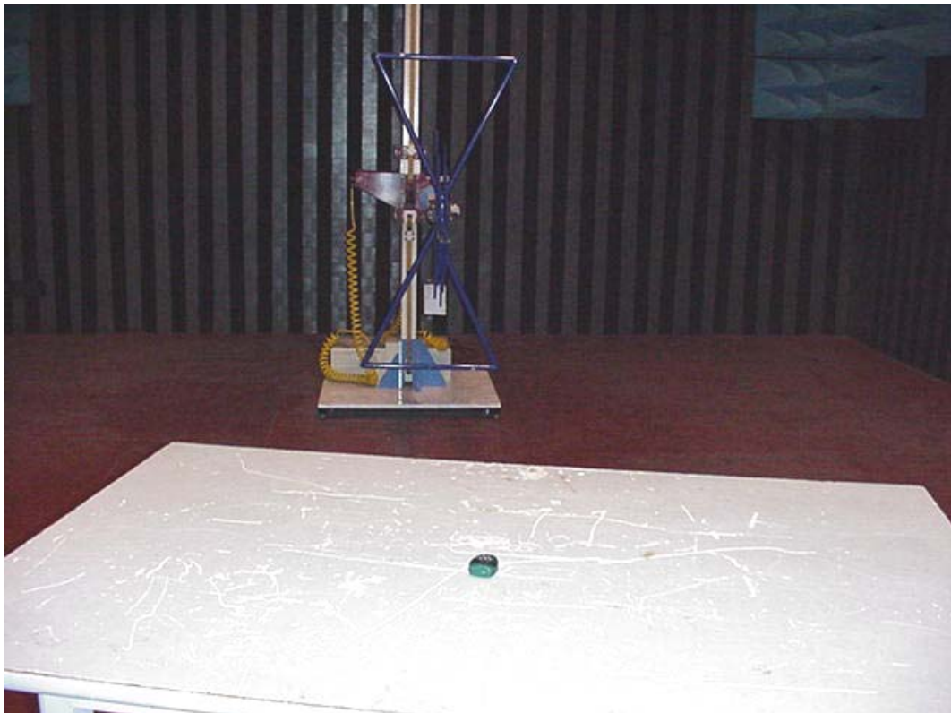
SETUP WITH MAXIMUM DETECTED EMISSION AT VERTICAL POLARIZATION (2 TEST MODE)
