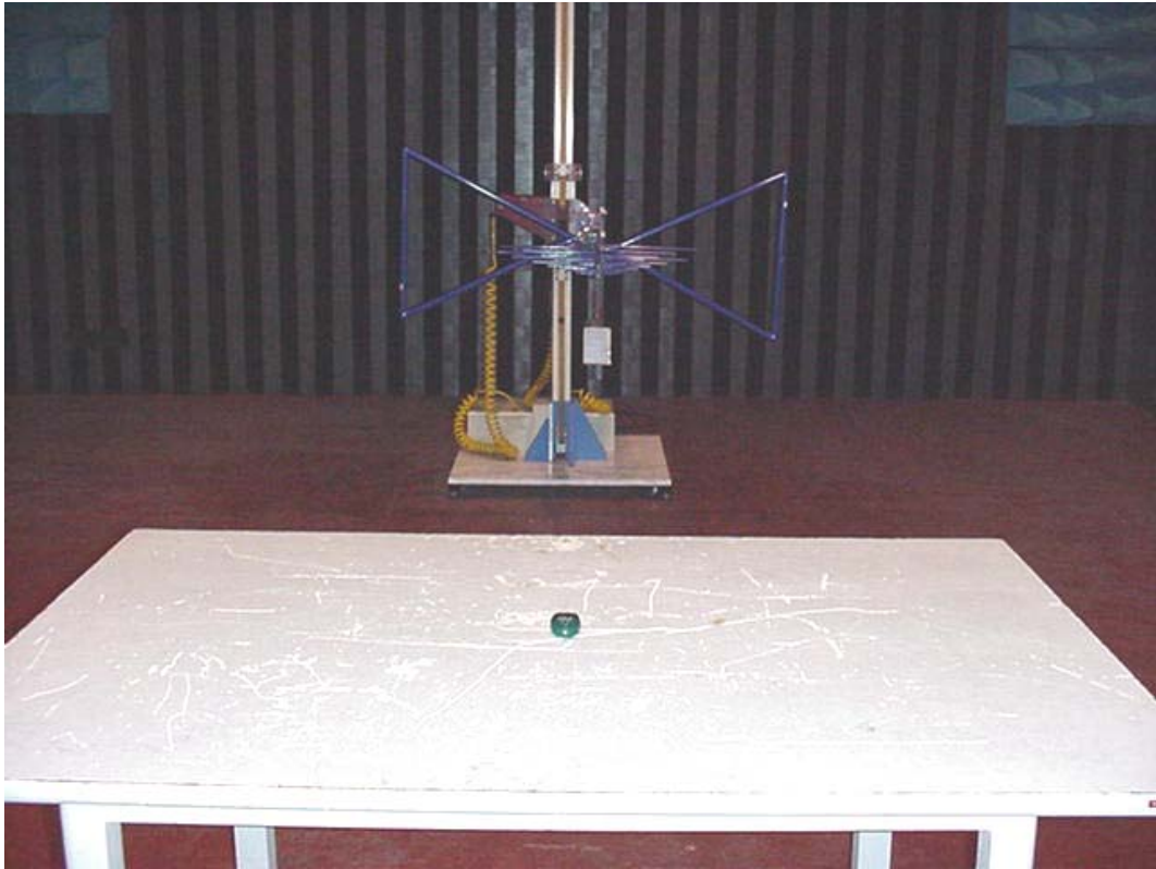
FRONT VIEW OF TEST (2 TEST MODE)
