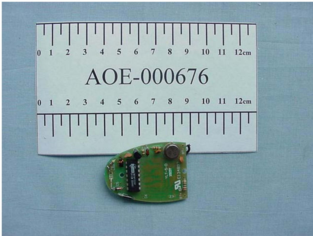
FIGURE 2 REMOTE CONTROLLER (M/N: YLT-5C) MAIN BOARD (COMPONENT SIDE)
