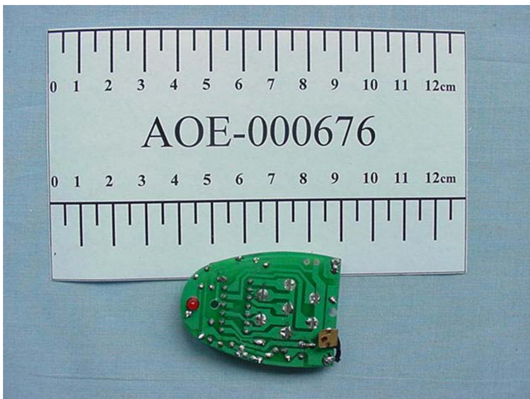
FIGURE 3 REMOTE CONTROLLER (M/N: YLT-5C) MAIN BOARD (SOLDERED SIDE)
