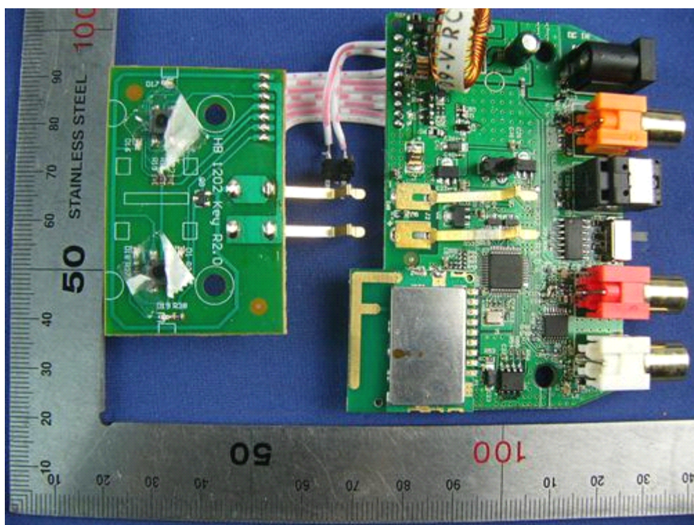
INTERNAL VIEW OF TX-3
