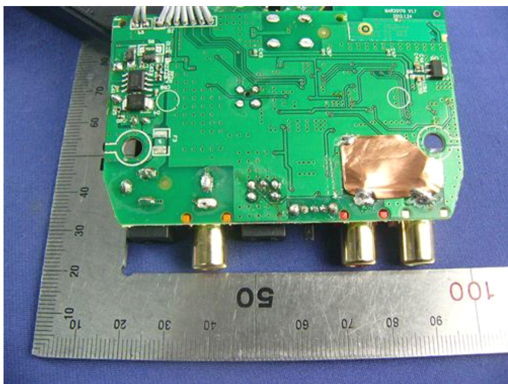
INTERNAL VIEW OF TX-4
