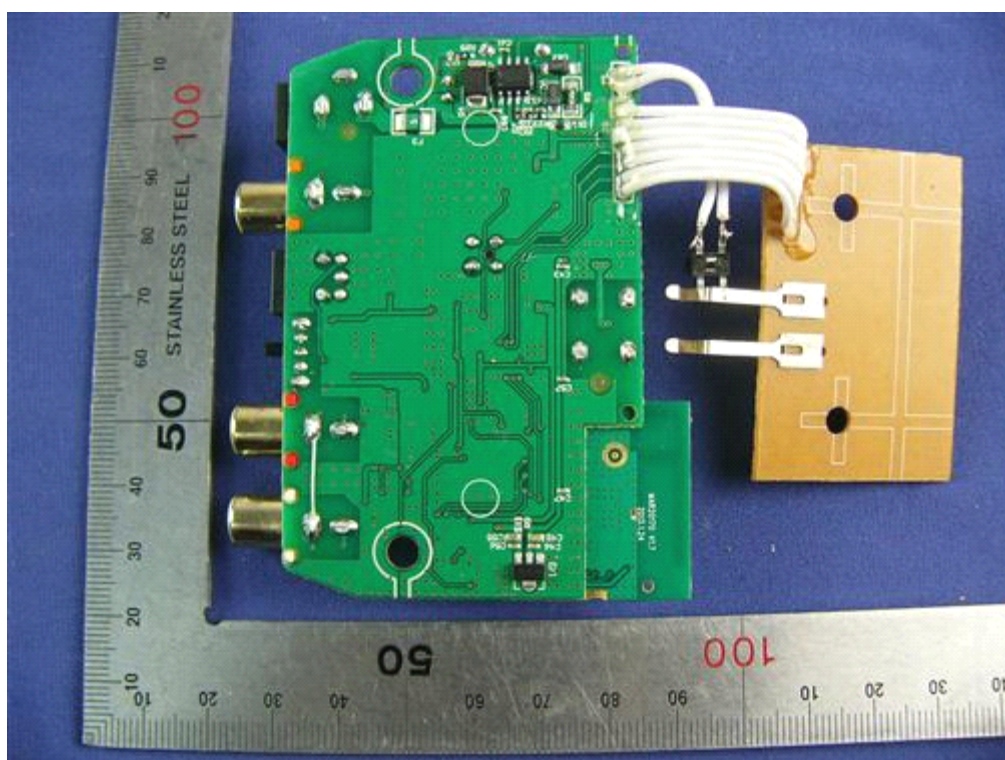
INTERNAL VIEW OF TX-5
