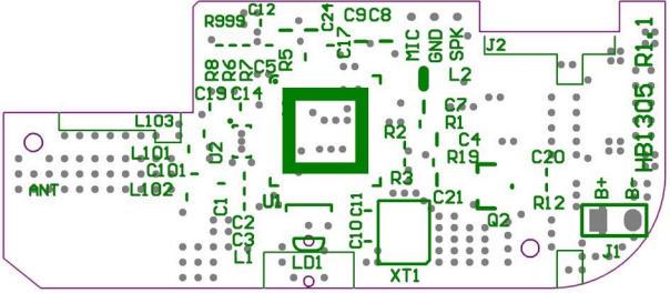
Top SilkScreen
