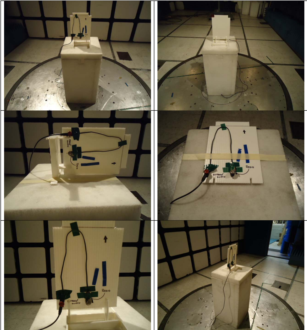
Conducted measurements setup
