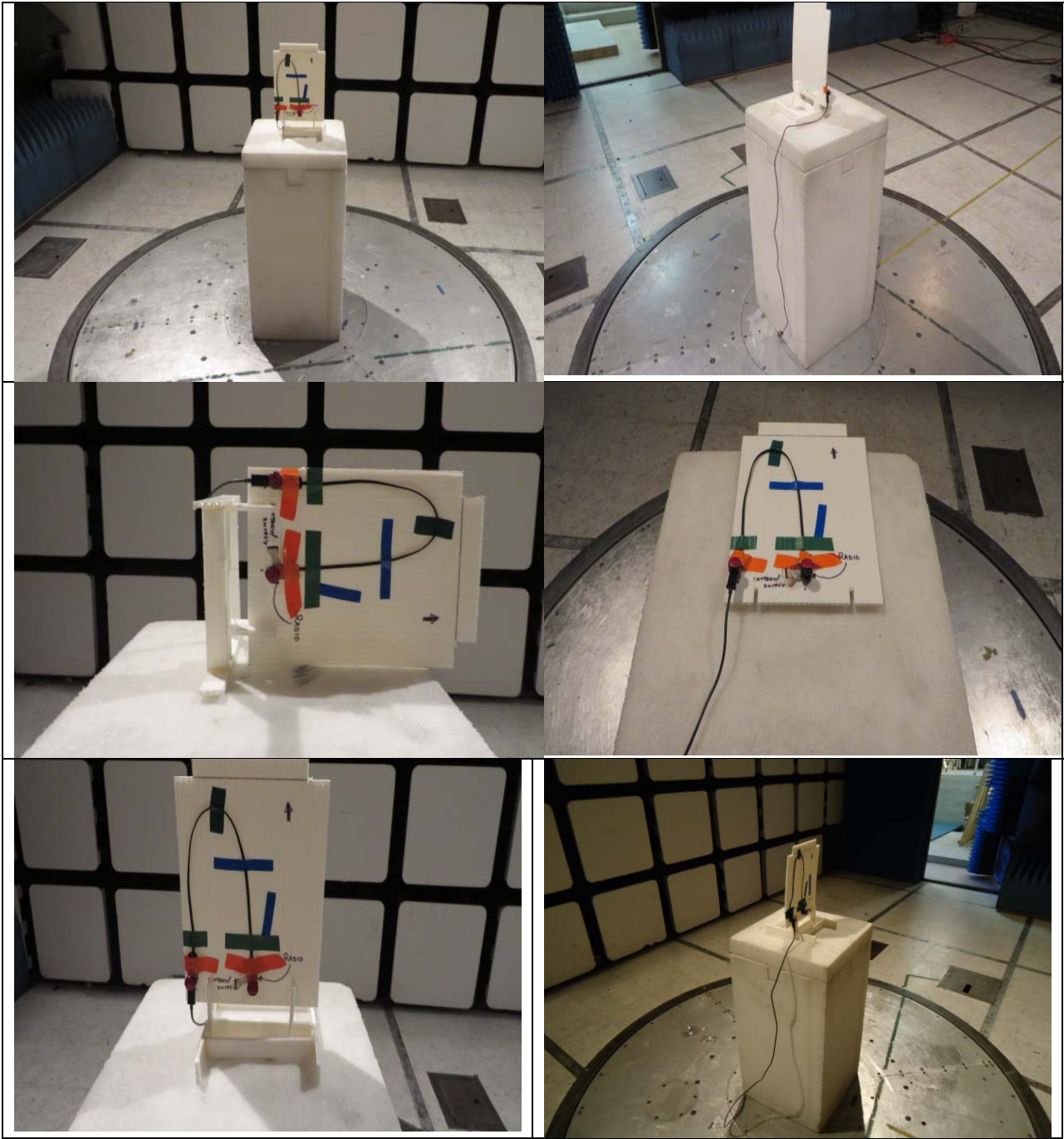
Radiated measurements setup
