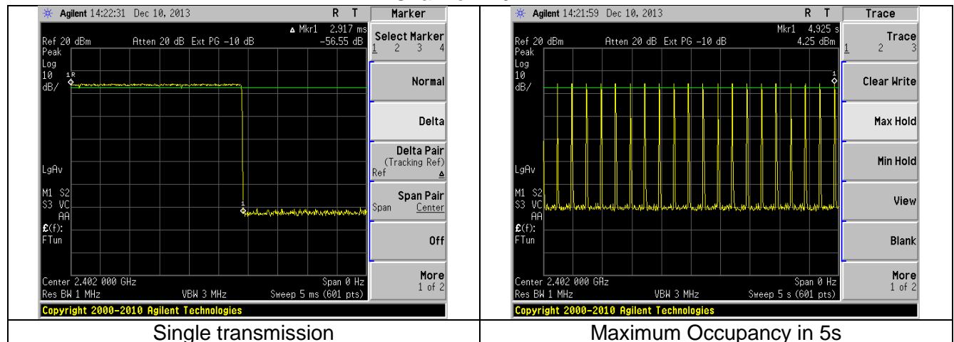
Channel 2402MHz
