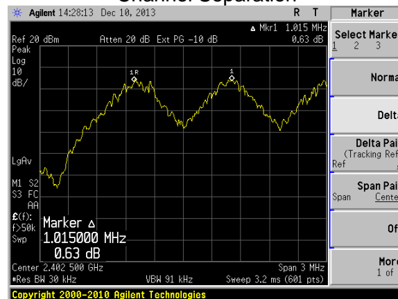
Channel Separation
