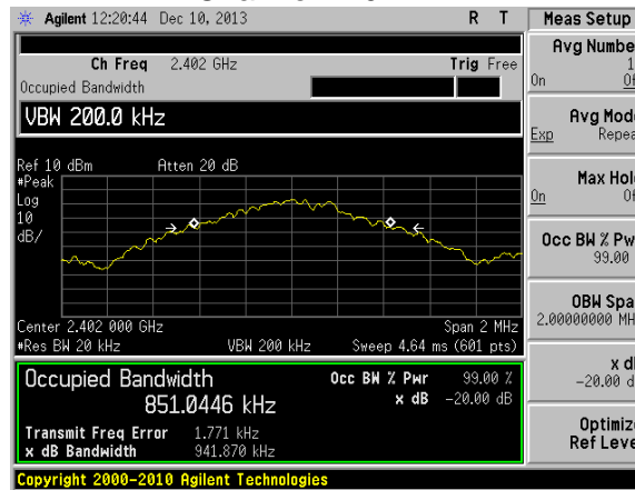
Channel 2402MHz
