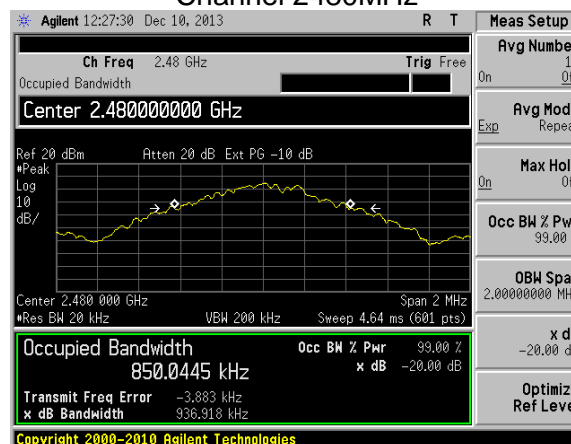
Channel 2480MHz
