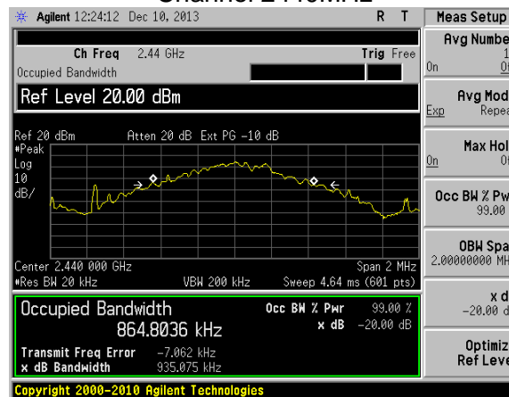
Channel 2440MHz
