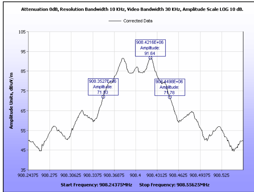
Plot 8. 908 MHz, Occupied Bandwidth
