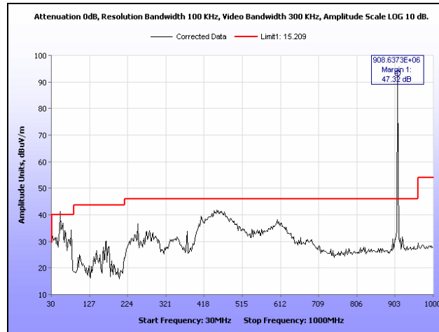
Plot 9. Radiated Spurious Emissions, 908 MHz, 30 MHz – 1 GHz
