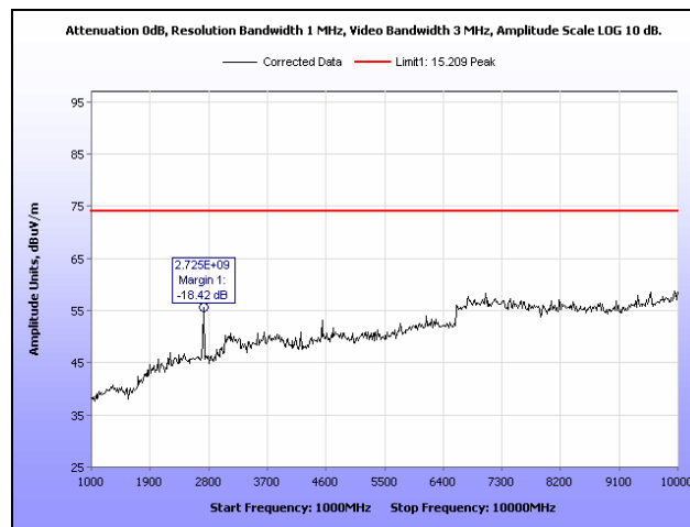
Plot 10. Radiated Spurious Emissions, 908 MHz, 1 GHz – 10 GHz, Peak
