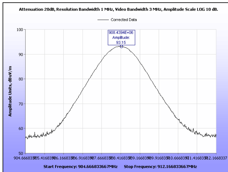
Plot 7. 908 MHz, Fundamental, TX, 30
