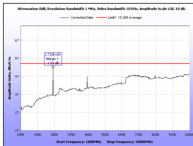
Plot 11. Radiated Spurious Emissions, 908 MHz, 1 GHz – 10 GHz, Average
