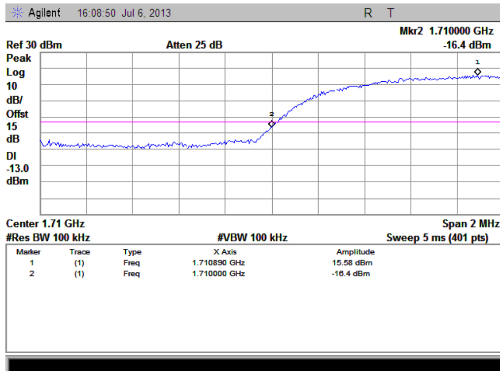
(Plot U: WCDMA 1700 Channel = 1312)
