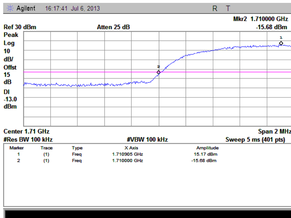
(Plot W : HSDPA 1700 Channel = 1312)
