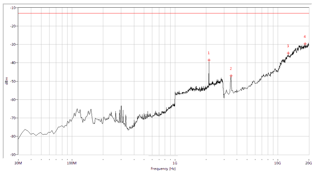
(Plot L.2: HSDPA 1700MHz Channel = 1312, Test Antenna Vertical)
