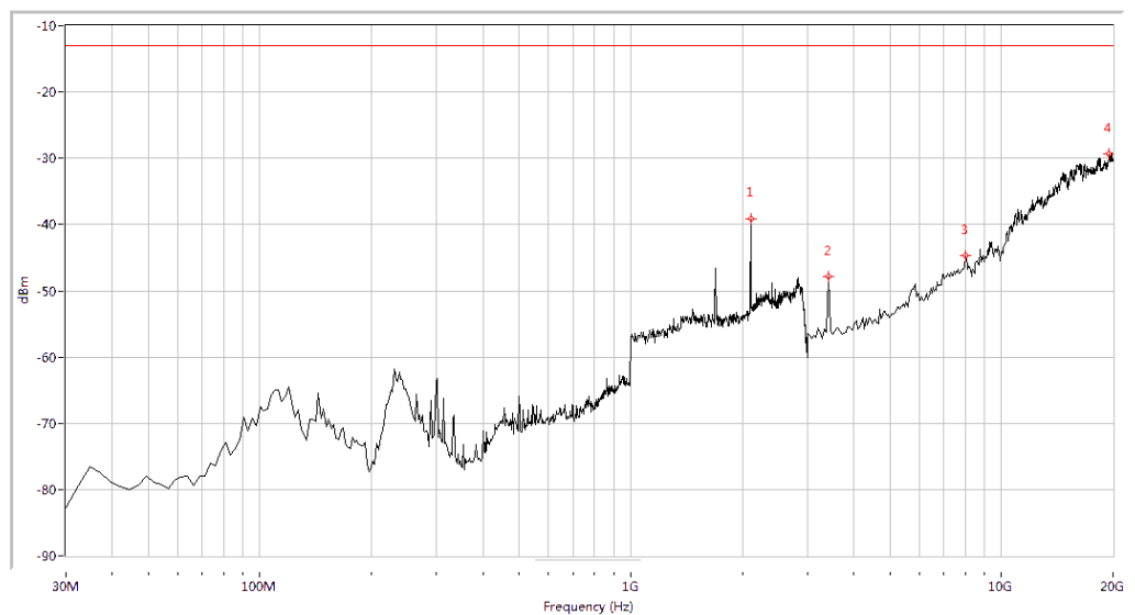
(Plot K.6: WCDMA 1700MHz Channel = 1513, Test Antenna Vertical)
