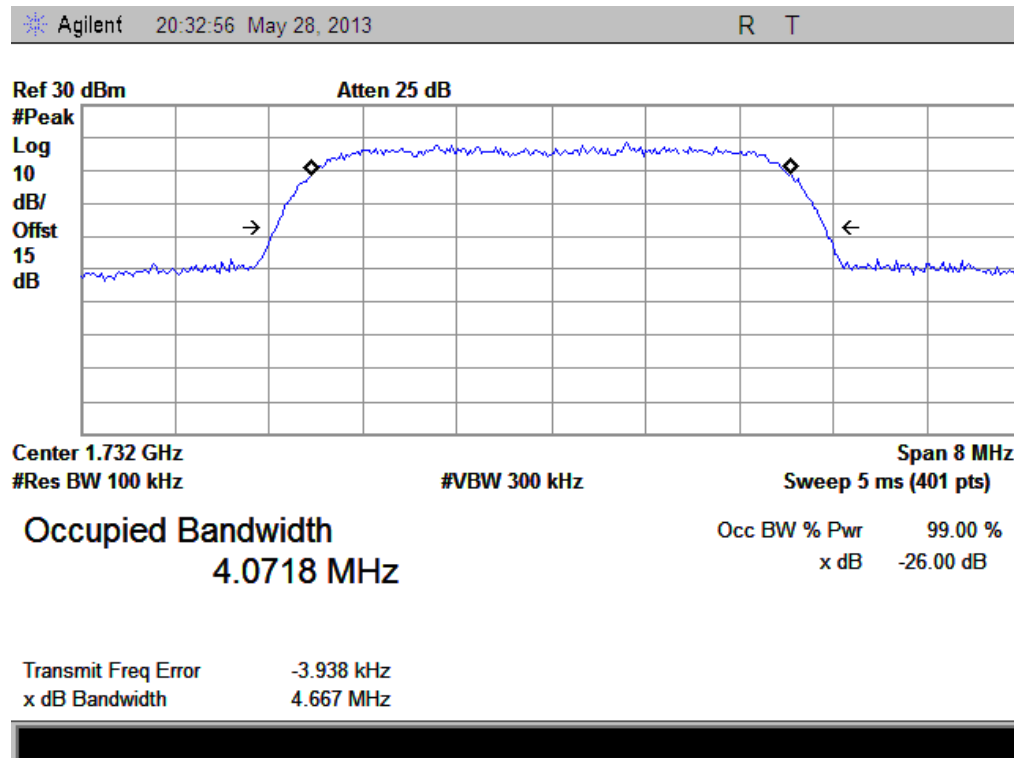
(Plot I1: HSDPA 1700 MHz Channel = 1412)
