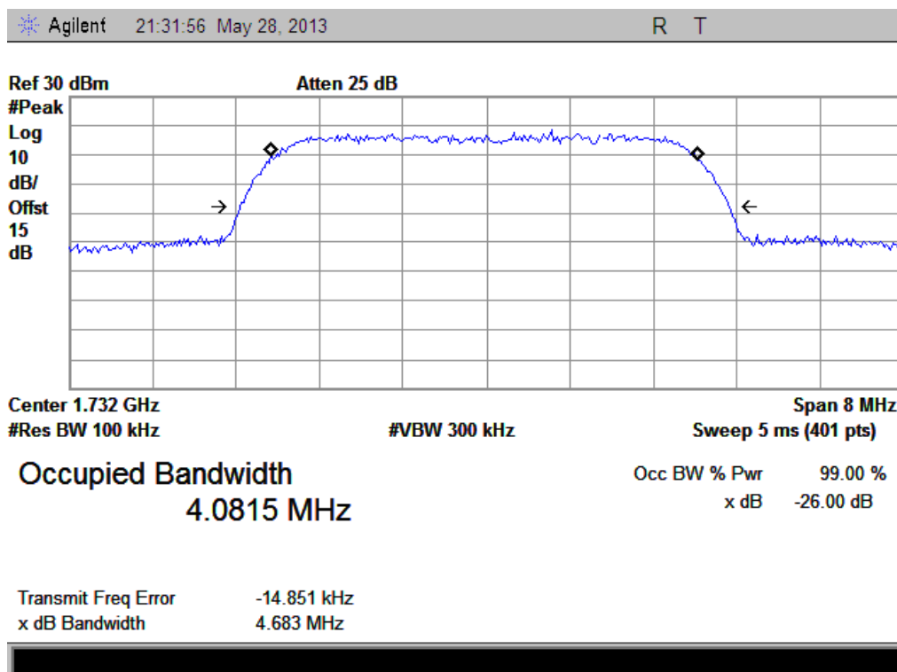
(Plot L1: HSUPA1700 MHz Channel = 1412)
