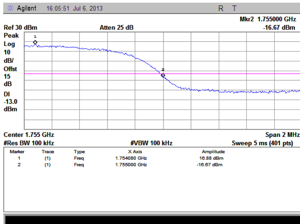
(Plot V: WCDMA 1700 Channel = 1513)
