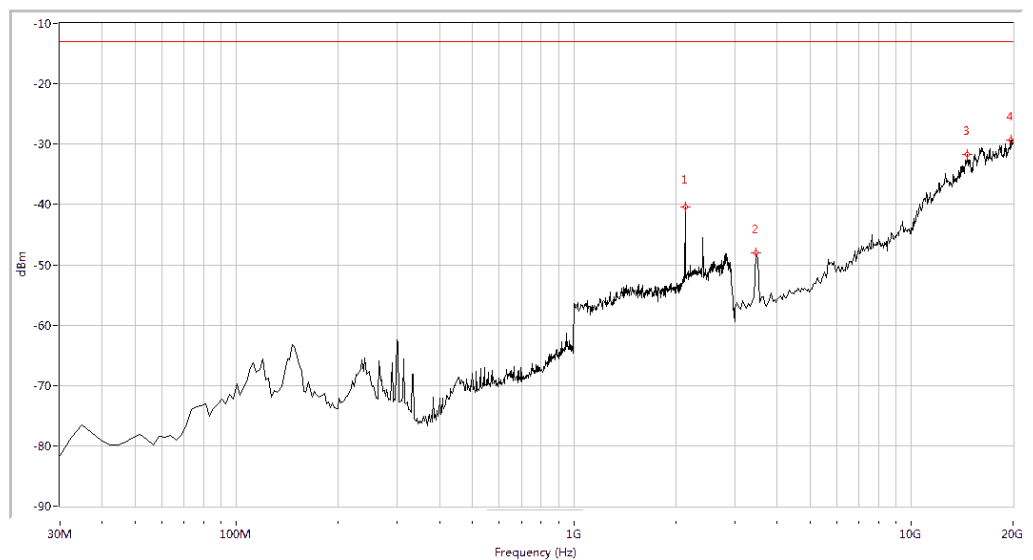
(Plot K.2: WCDMA 1700MHz Channel = 1312, Test Antenna Vertical)
