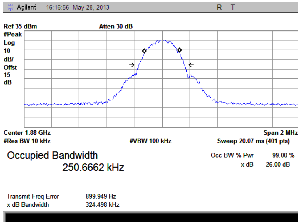
(Plot C1: GSM 1900MHz Channel = 661)
