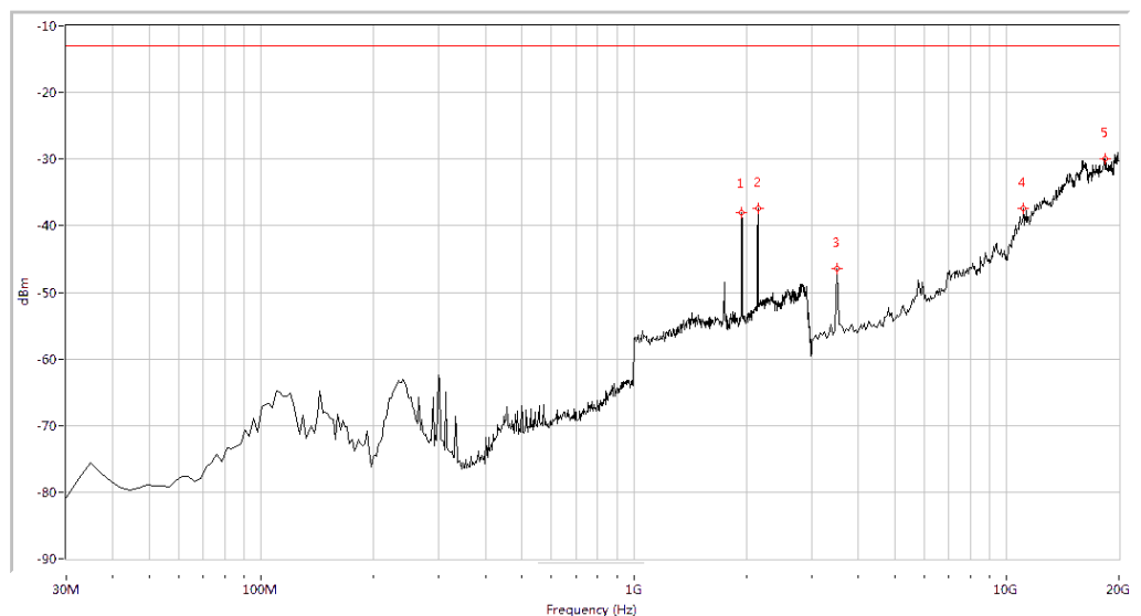
(Plot K.4: WCDMA 1700MHz Channel = 1412, Test Antenna Vertical)
