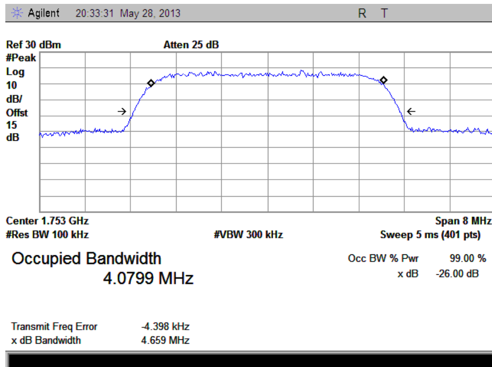
(Plot J1: HSDPA 1700MHz Channel = 1513)
