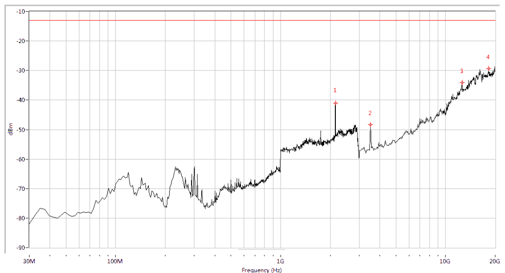
(Plot L.4: HSDAP 1700MHz Channel = 1412, Test Antenna Vertical)
