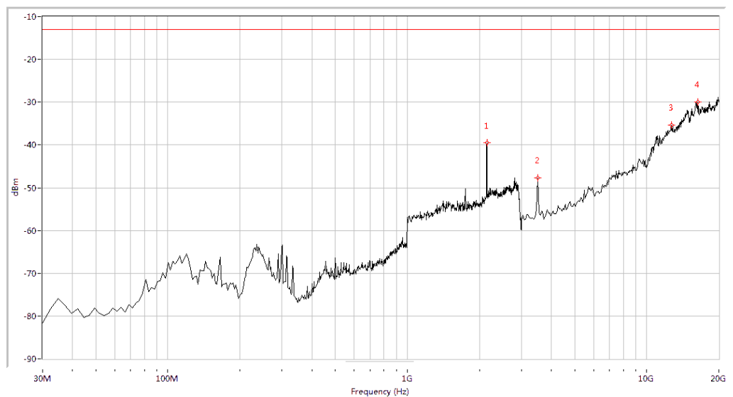
(Plot M.4: HSUPA 1700MHz Channel =1412, Test Antenna Vertical)
