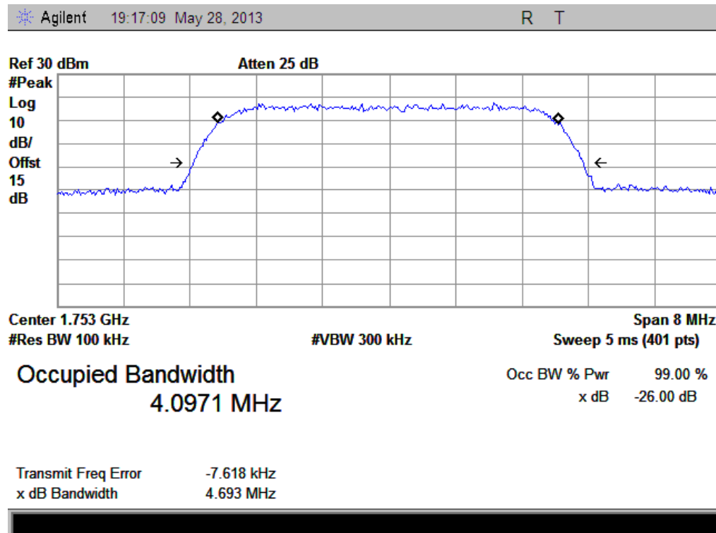
(Plot G1: WCDMA 1700MHz Channel = 1513)
