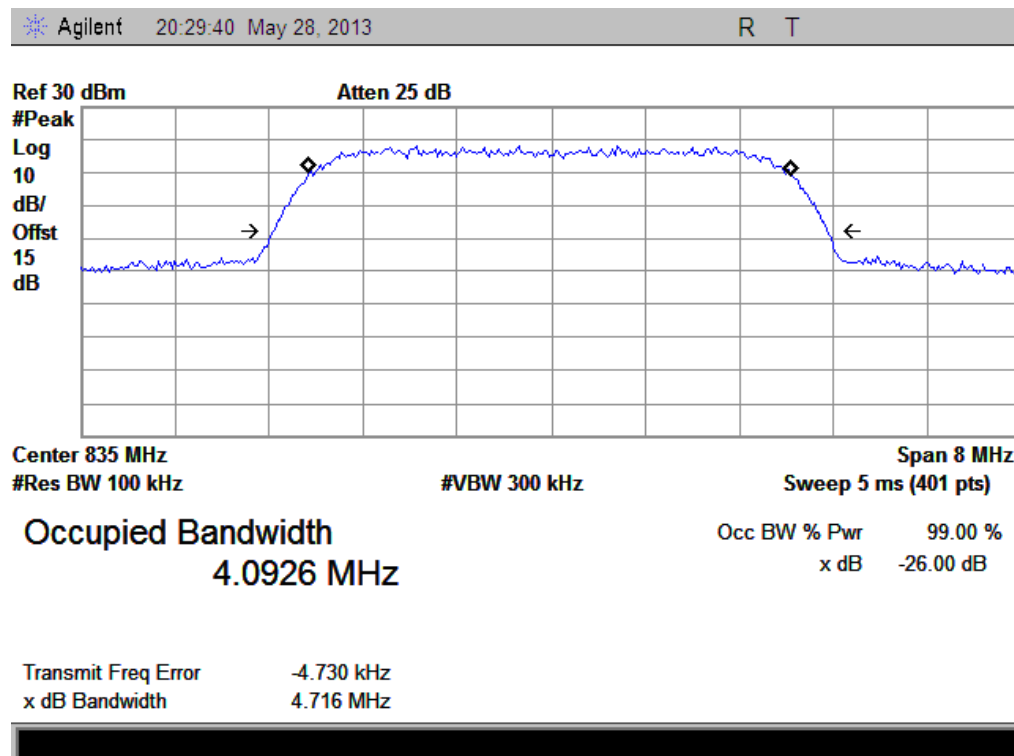
(Plot N: HSDPA850 MHz Channel = 4175)
