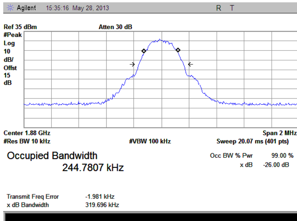
(Plot R1: GPRS 1900MHz Channel = 661)
