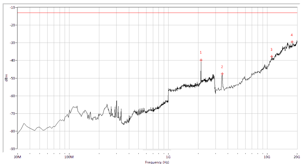
(Plot M.2: HSUPA 1700MHz Channel = 1312, Test Antenna Vertical)
