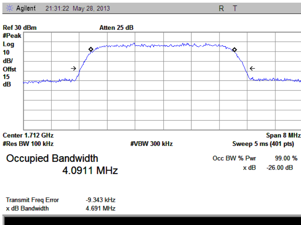
(Plot K1: HSUPA 1700MHz Channel = 1312)
