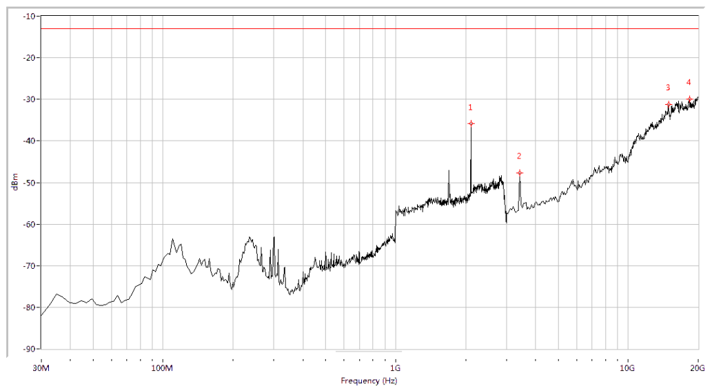
(Plot L.6: HSDPA 1700MHz Channel = 1513, Test Antenna Vertical)
