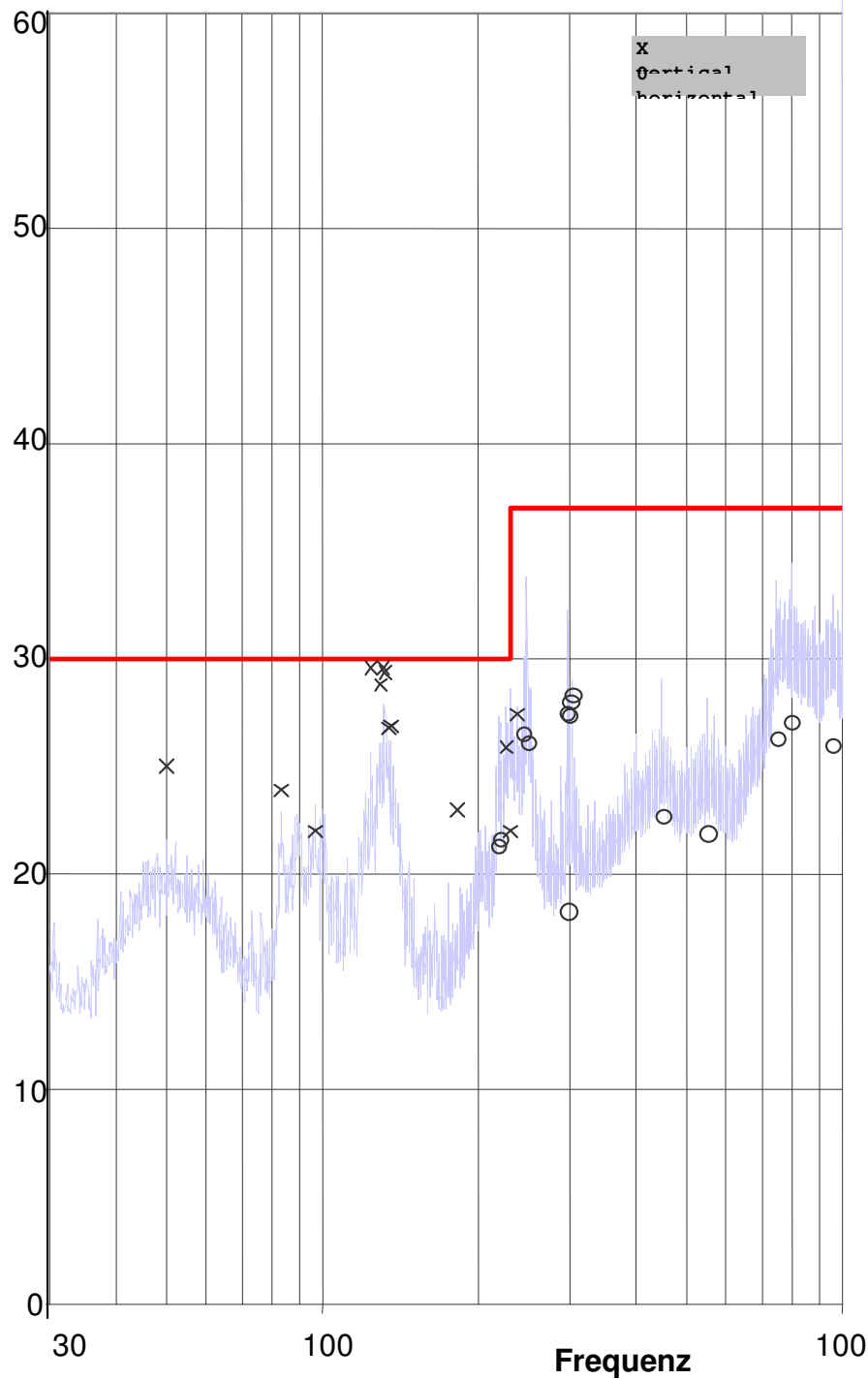
graph 5.1: radiated emission
