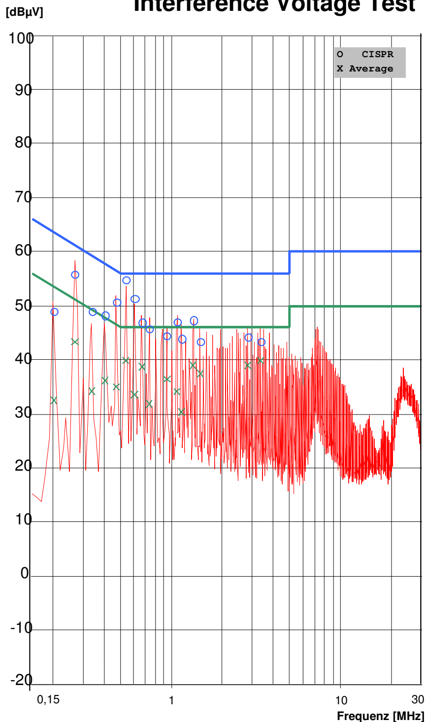
graph 4.1: conducted emission at line 1
