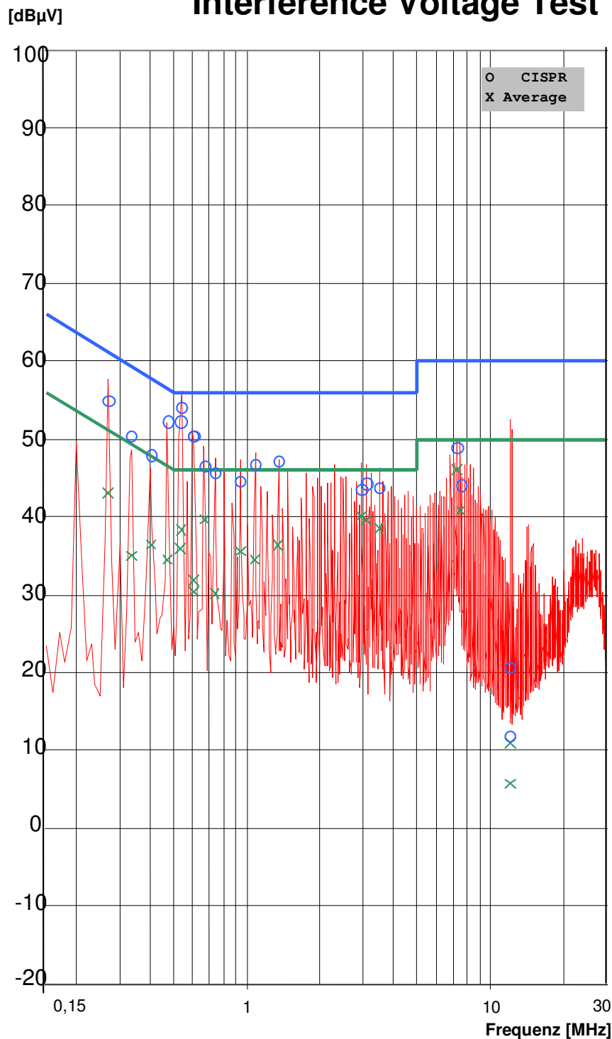
graph 4.2: conducted emission at line 2
