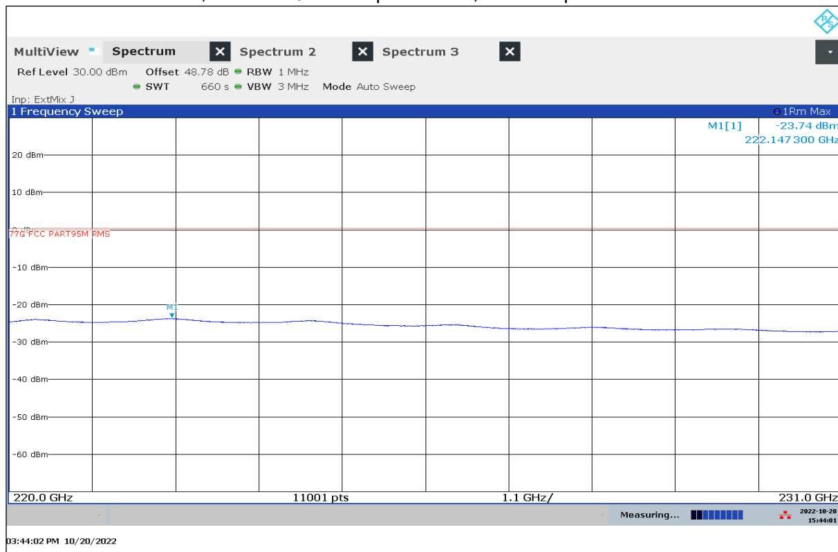
Plot 18: 220 GHz to 231 GHz, horizontal / vertical polarization, valid for specified modes
