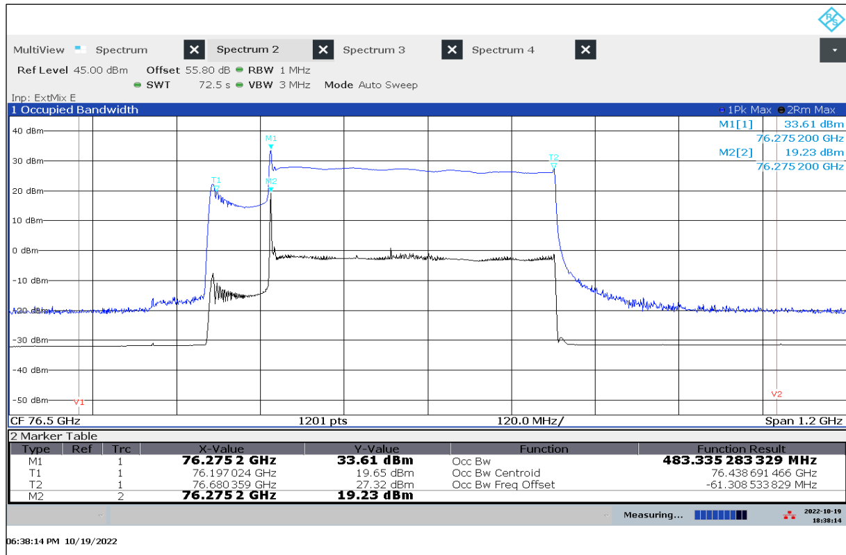
Plot 27: OBW, +50 °C / V_{nom}
