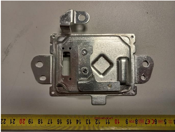
REAR HOUSING – SIDE 1
