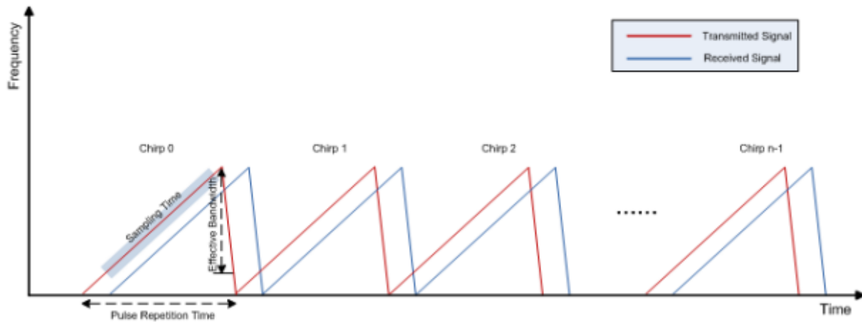
Figure 3: Chirp timing
