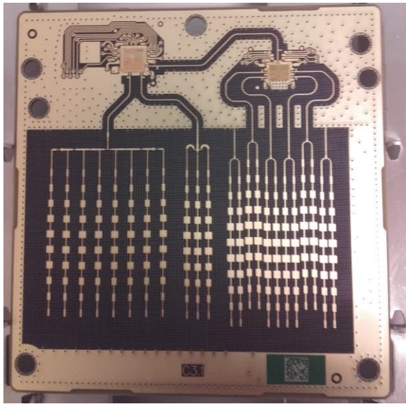
Antenna PCB - Side 1
