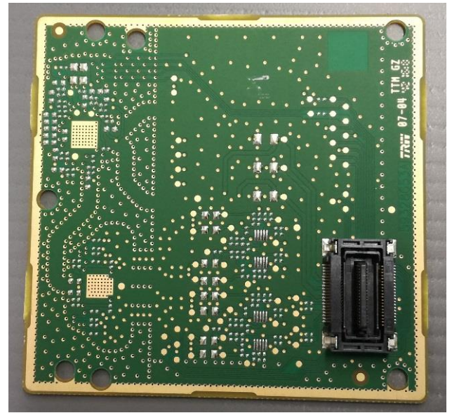
Antenna PCB - Side 2
