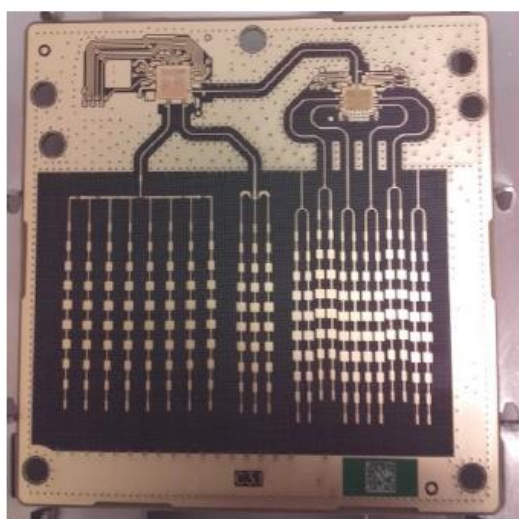
Antenna PCB - Side 1
