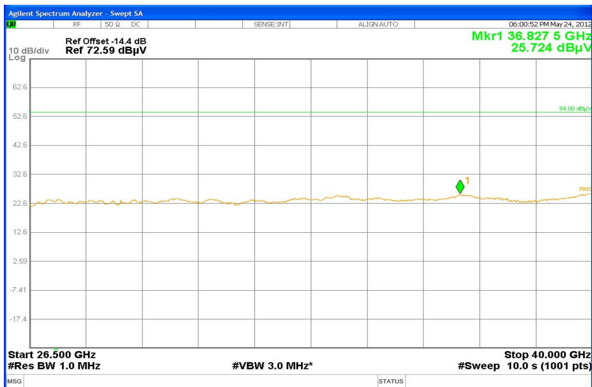
Plot No. 18: 26.5 GHz to 40 GHz, horizontal / vertical polarization, low/mid/high frequency
