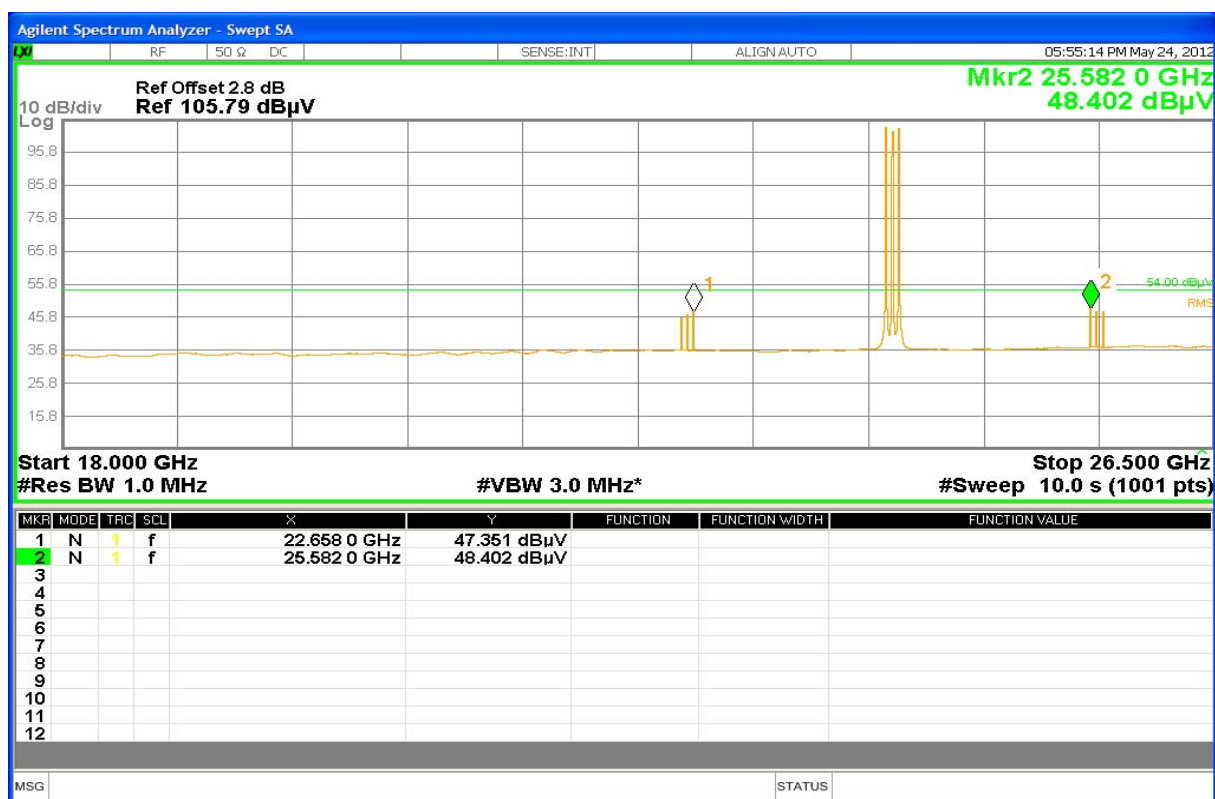
Plot No. 17: 18 GHz to 26.5 GHz, horizontal / vertical polarization, low/mid/high frequency
