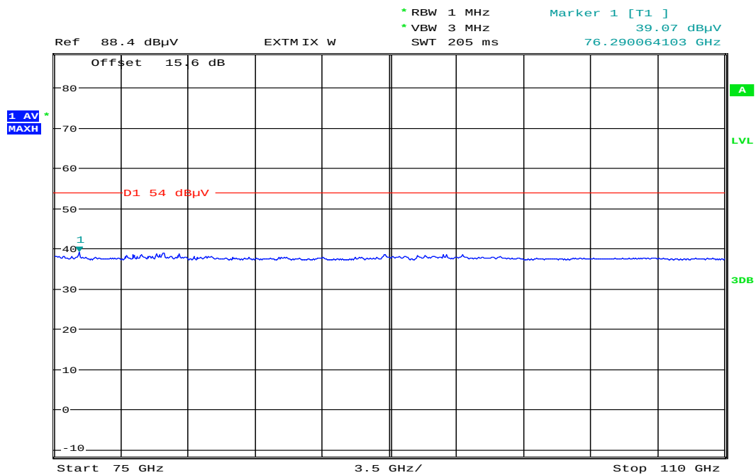
Plot No. 22: 75 GHz to 110 GHz, horizontal / vertical polarization, mid frequency
