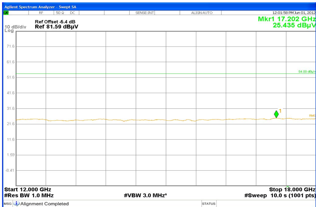
Plot No. 16: 12 GHz to 18 GHz, horizontal / vertical polarization, low/mid/high frequency
