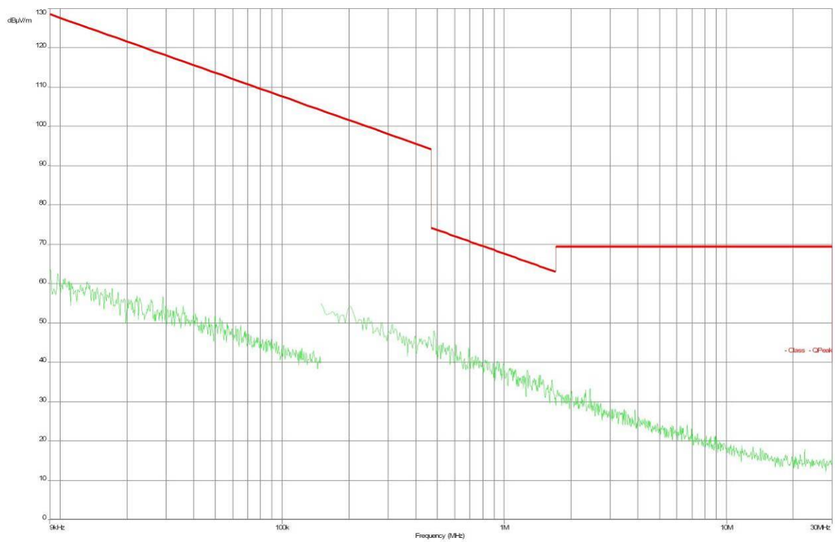
Plot No. 9: Magnetic, TX mode up to 30 MHz (Valid for all frequencies)
