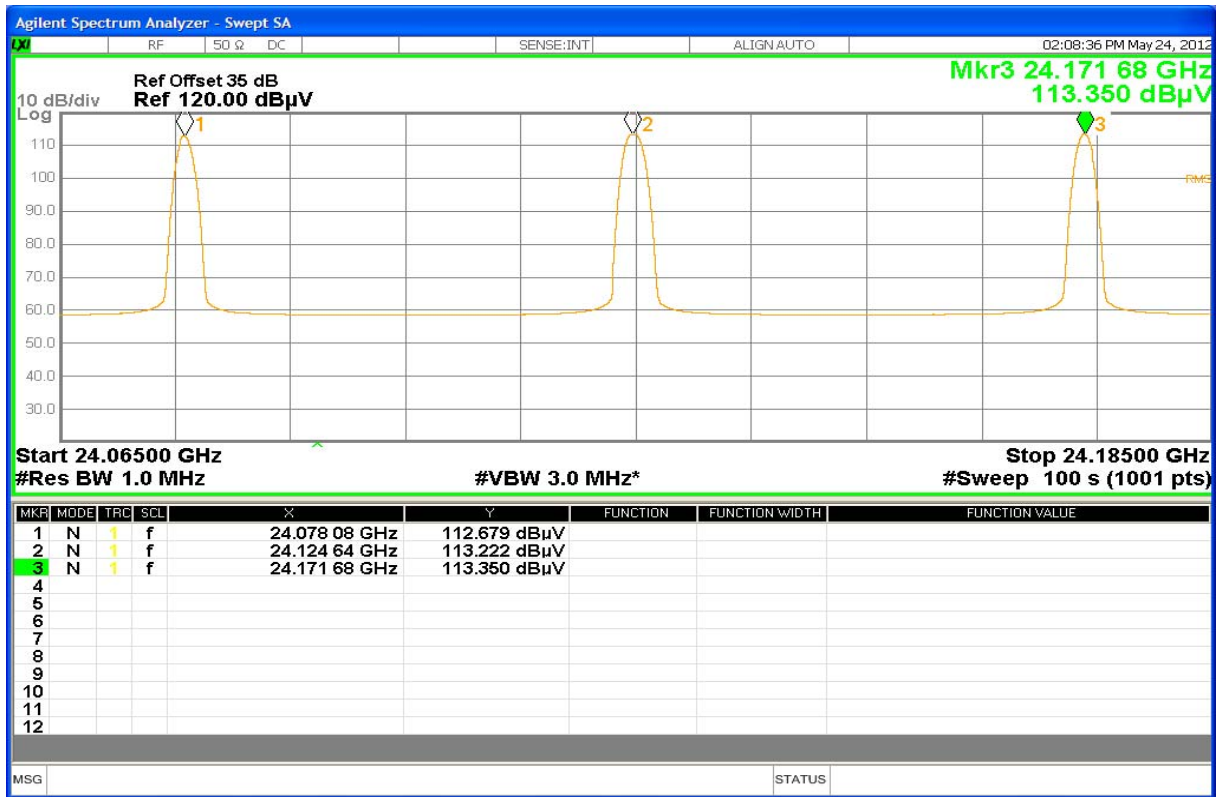
Plot No. 3: Stopped mode (low, middle, high frequency), Average-Measurement, T_{nom} / V_{nom}
