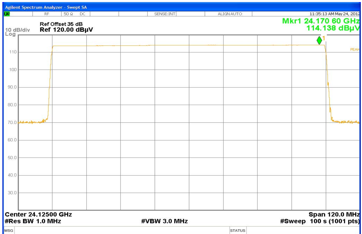
Plot No. 2: Normal operation mode, Peak-Measurement, T_{nom} / V_{nom}
