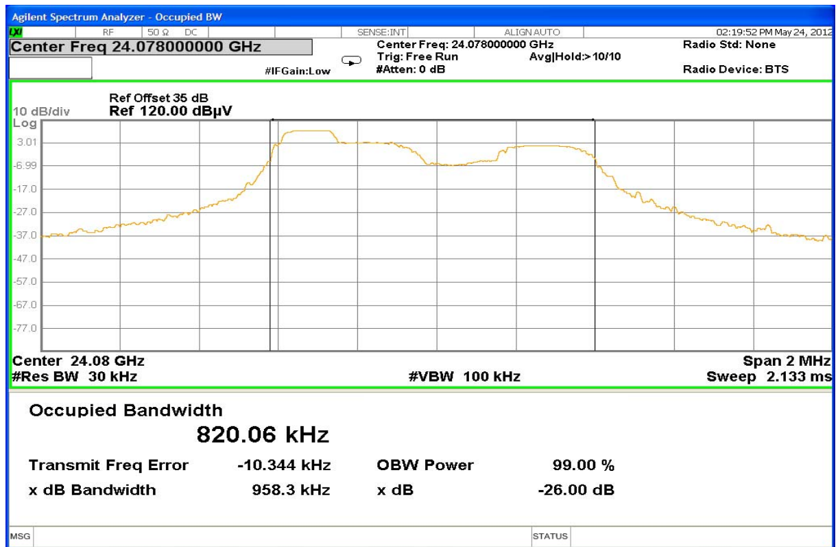
Plot No. 6: stopped mode, low frequency
