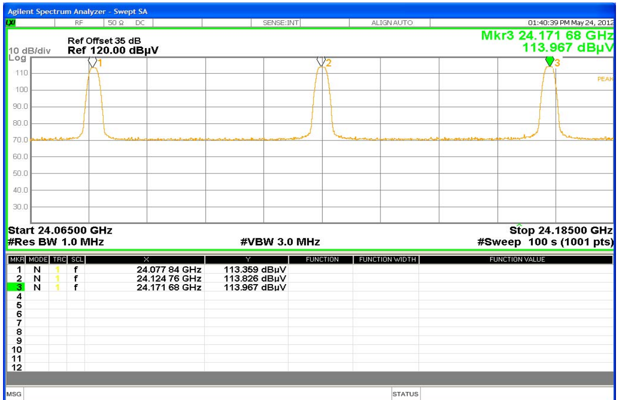
Plot No. 4: Stopped mode (low, middle, high frequency), Peak-Measurement, T_{nom} / V_{nom}
