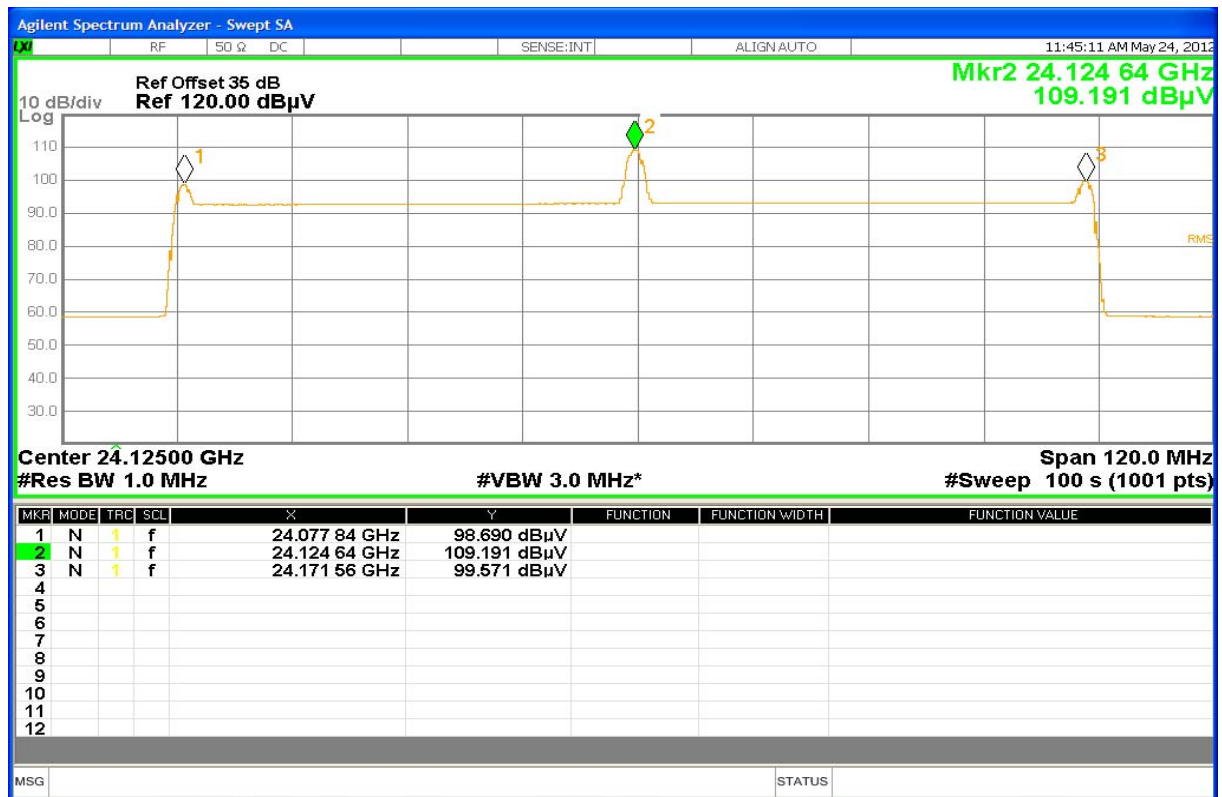
Plot No. 1: Normal operation mode, Average-Measurement, T_{nom} / V_{nom}
