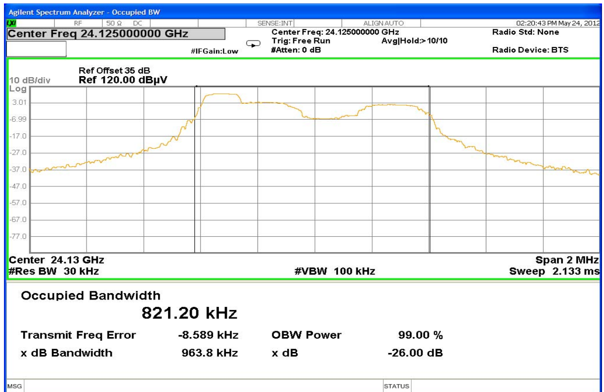
Plot No. 7: stopped mode, mid frequency
