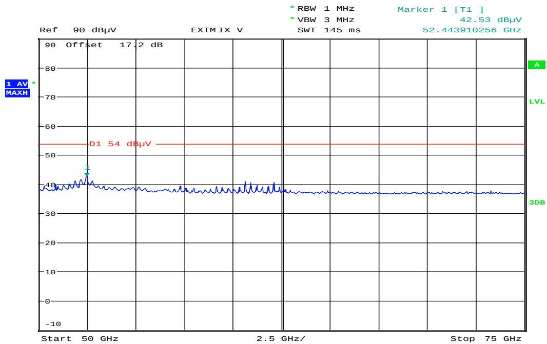
Plot No. 21: 50 GHz to 75 GHz, horizontal / vertical polarization, low frequency
