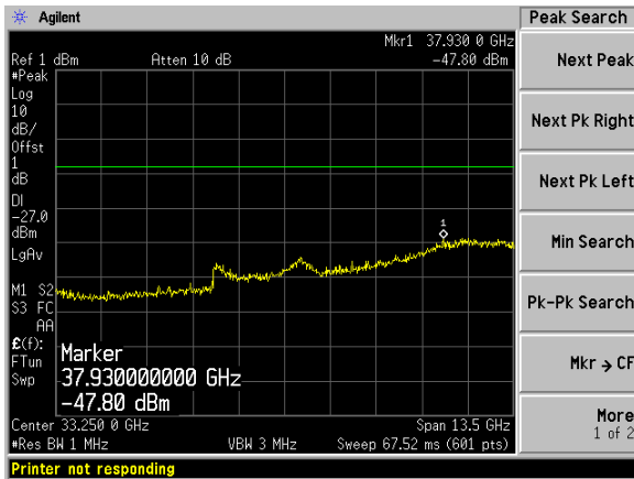
Chain 1, Plot: 26 GHz – 40 GHz
