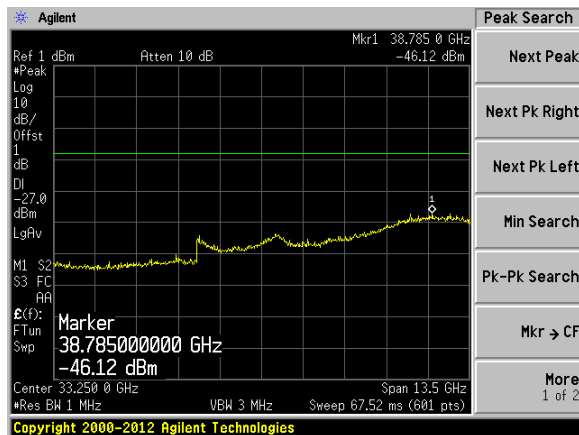
Chain 0, Plot: 26 GHz – 40 GHz
