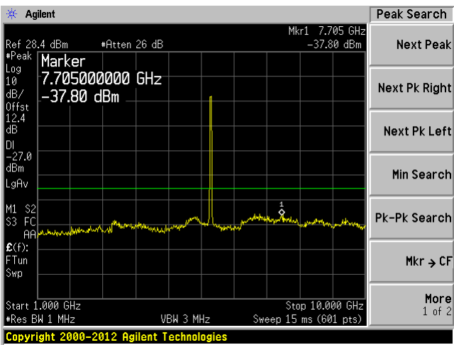
Chain 1 1GHz—10GHz
