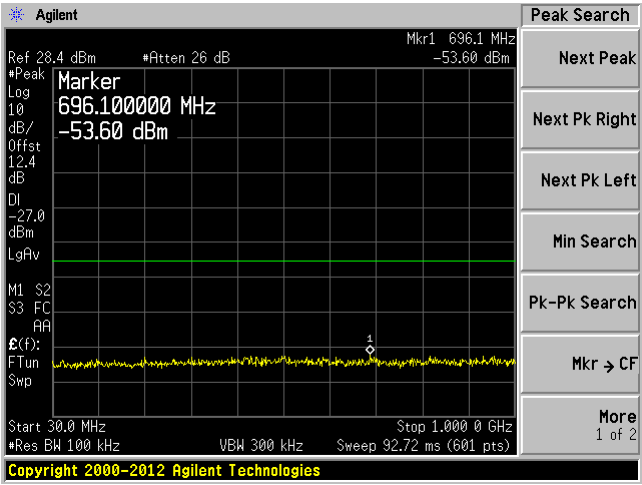
Chain 1 30MHz---1GHz
