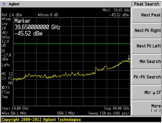
Chain 1 10GHz---40GHz
