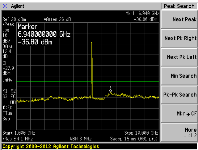
Chain 0 1GHz---10GHz
