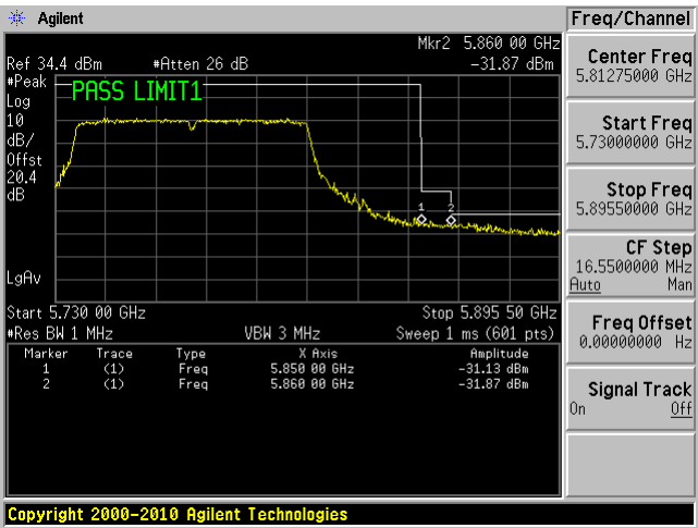
Chain 1 Higher Band Edge
