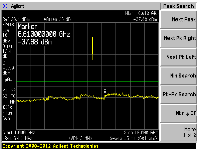
Chain 1 1GHz—10GHz
